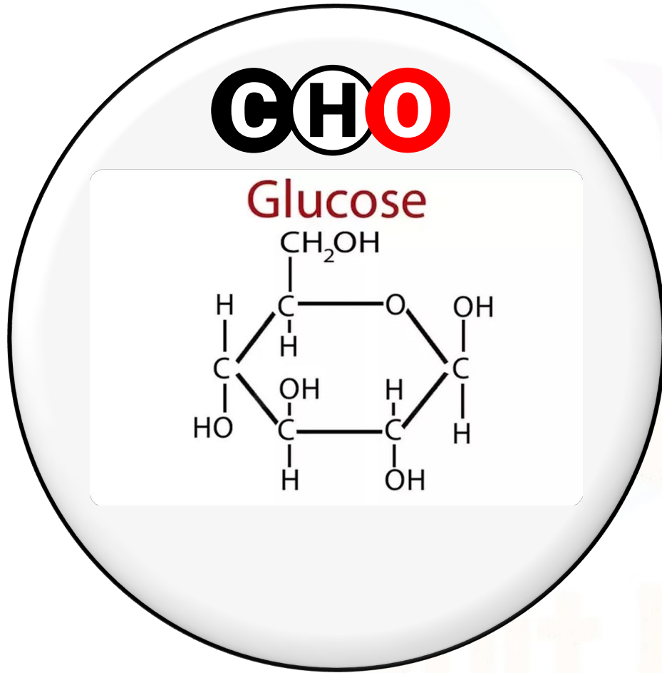
Monosaccharides
