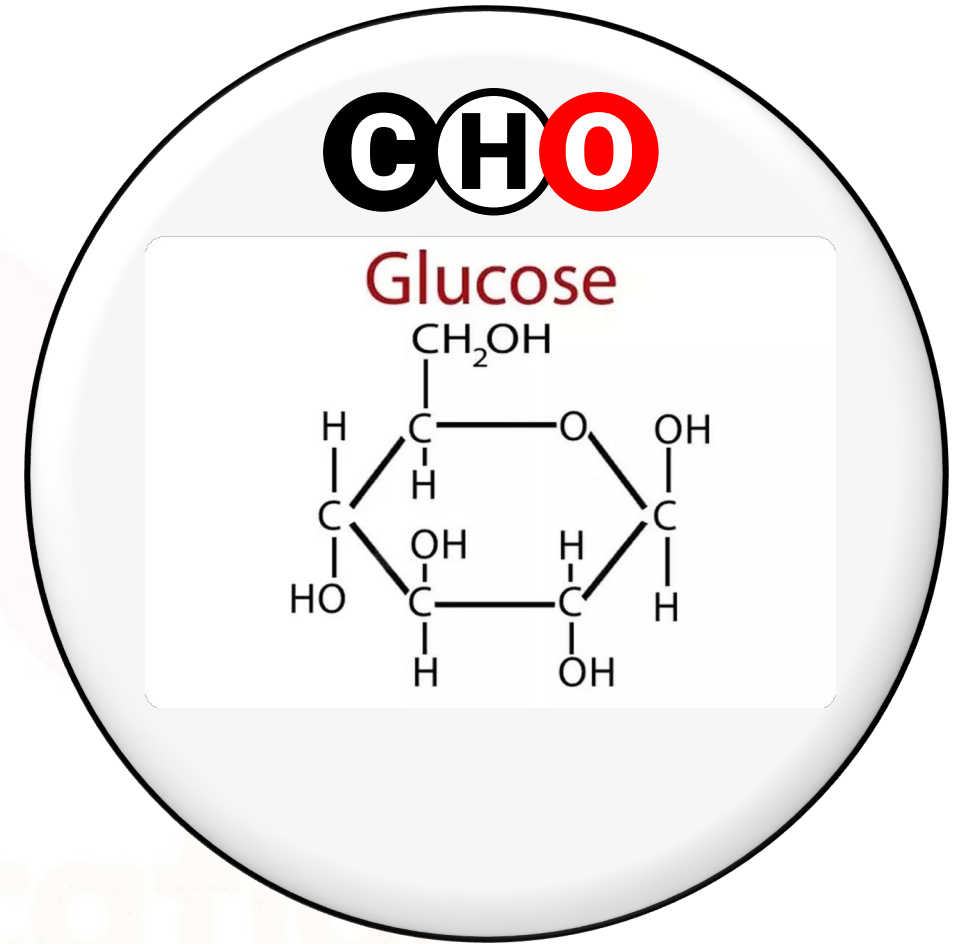
Monosaccharides
