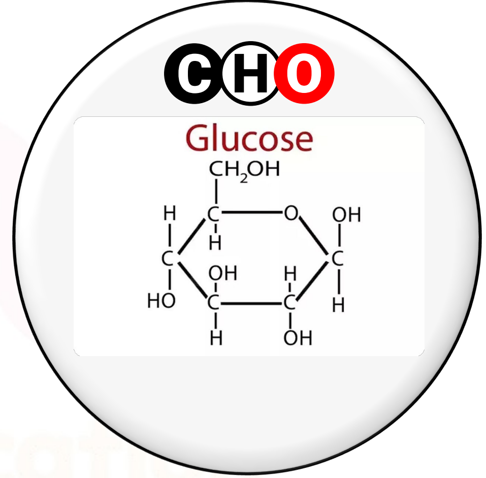
Monosaccharides
