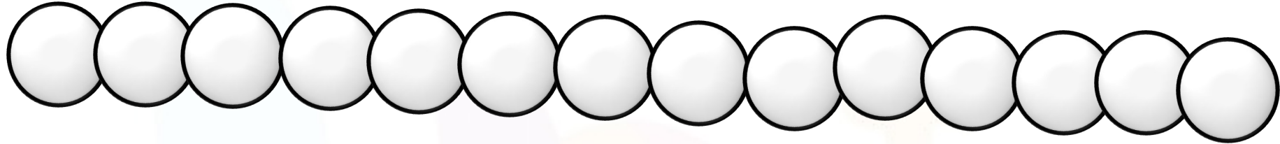
Polypeptide chain 1
