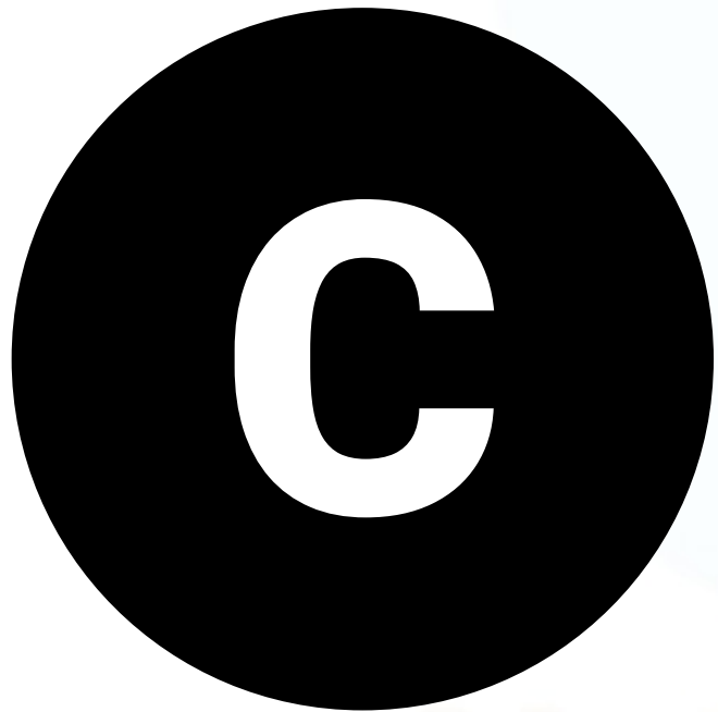
Carbon
