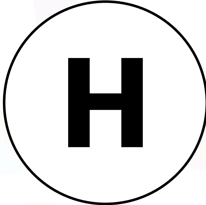
Hydrogen
