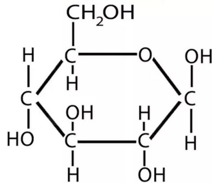
Glucose
