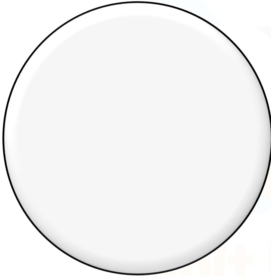
Mono(單)-mer
