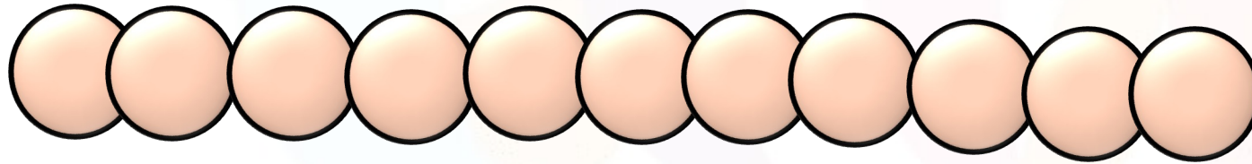
Polypeptide chain 2
