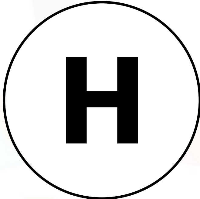
Hydrogen
