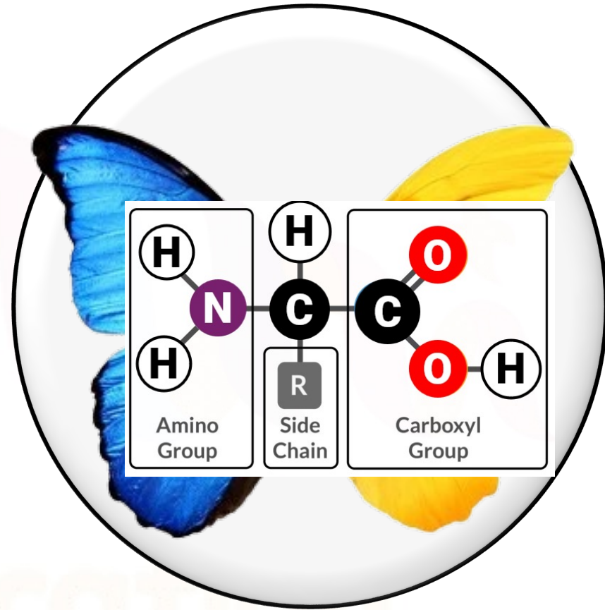
Amino acid
