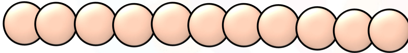
Polypeptide chain 2
