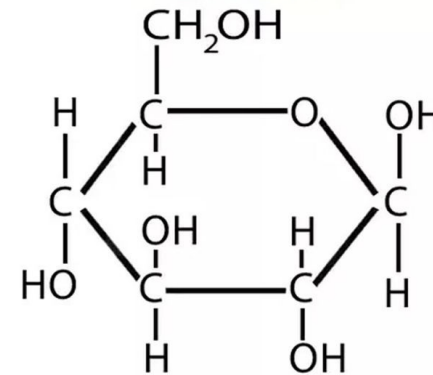
Glucose
