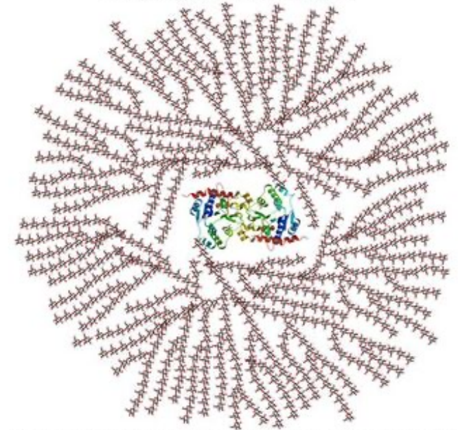
Glycogen structure
