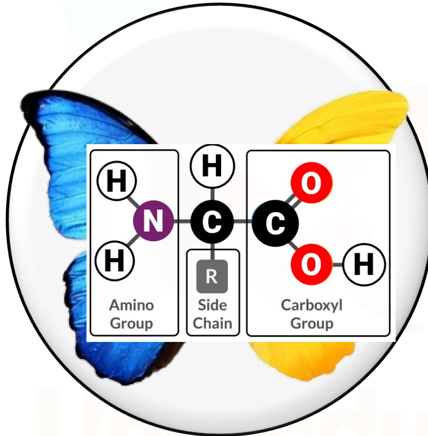
Amino acid
