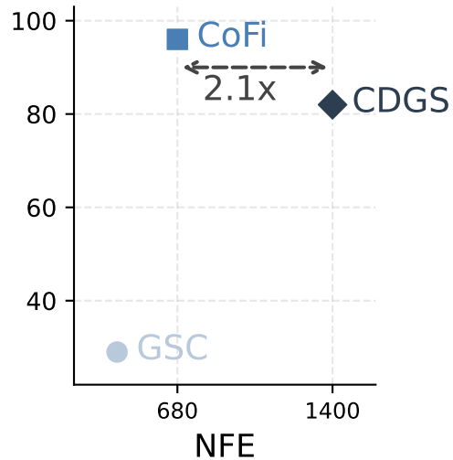
Success Rate (%)
