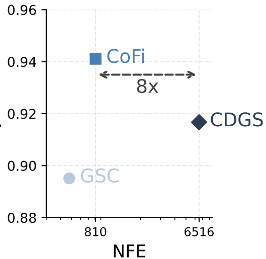
Subject ↑
