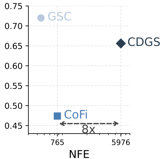
Intra-LPIPS ↓
