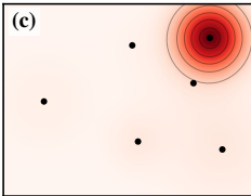
Inverse KKT
