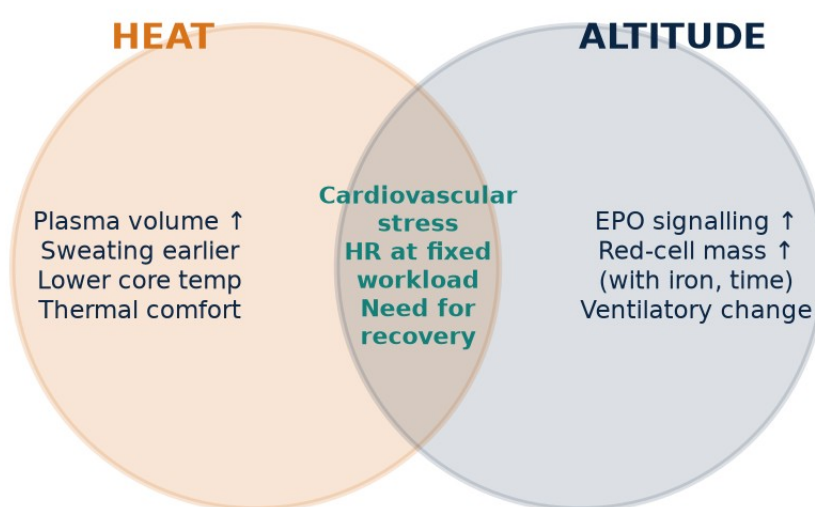
Figure 14. Heat and altitude overlap in cardiovascular stress but have different primary adaptations. Define the target adaptation before choosing the environment.
