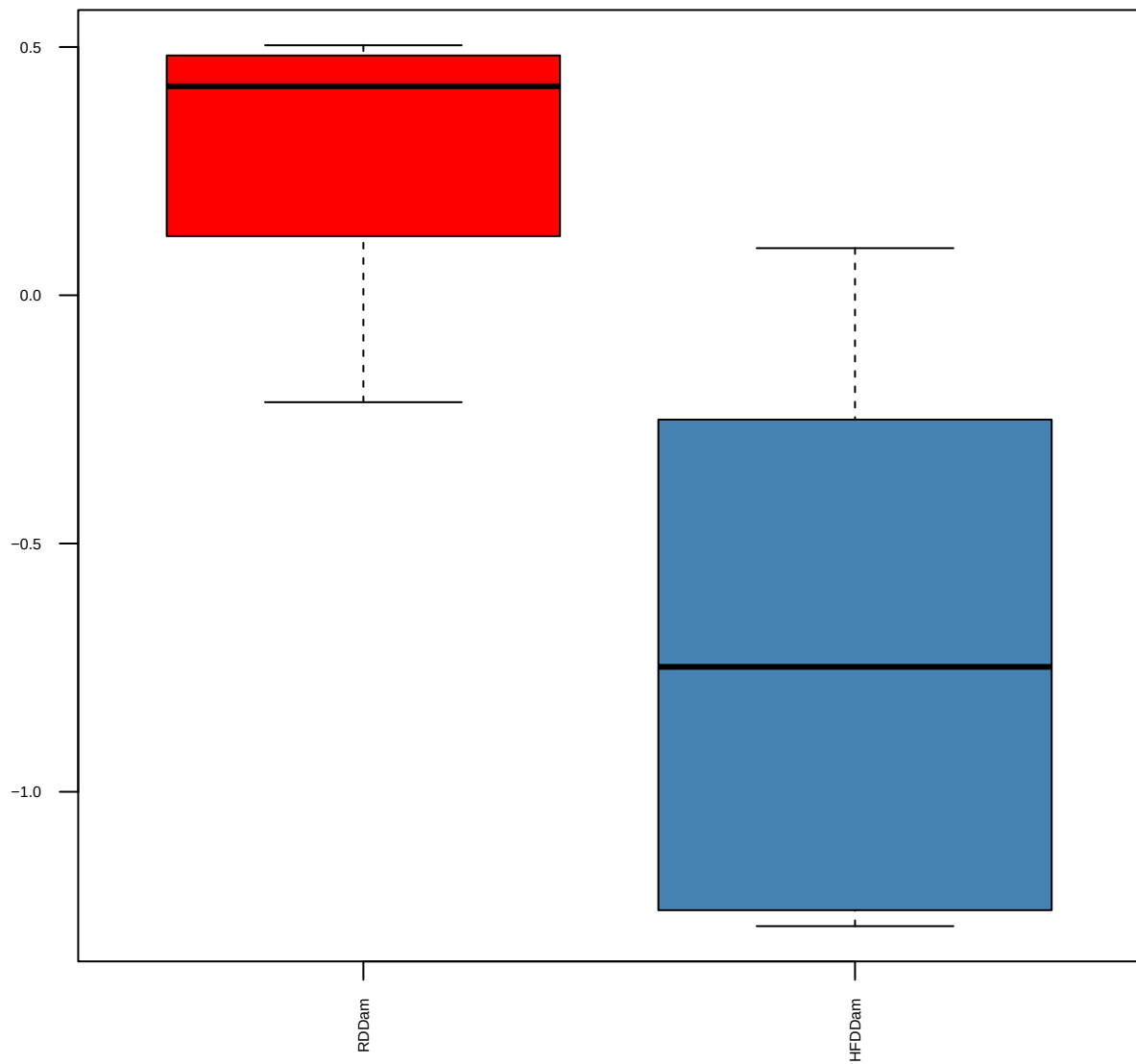
Cystine (FDR = 0.01)
