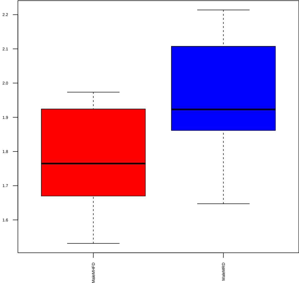
Histidine (FDR = 0.36)
