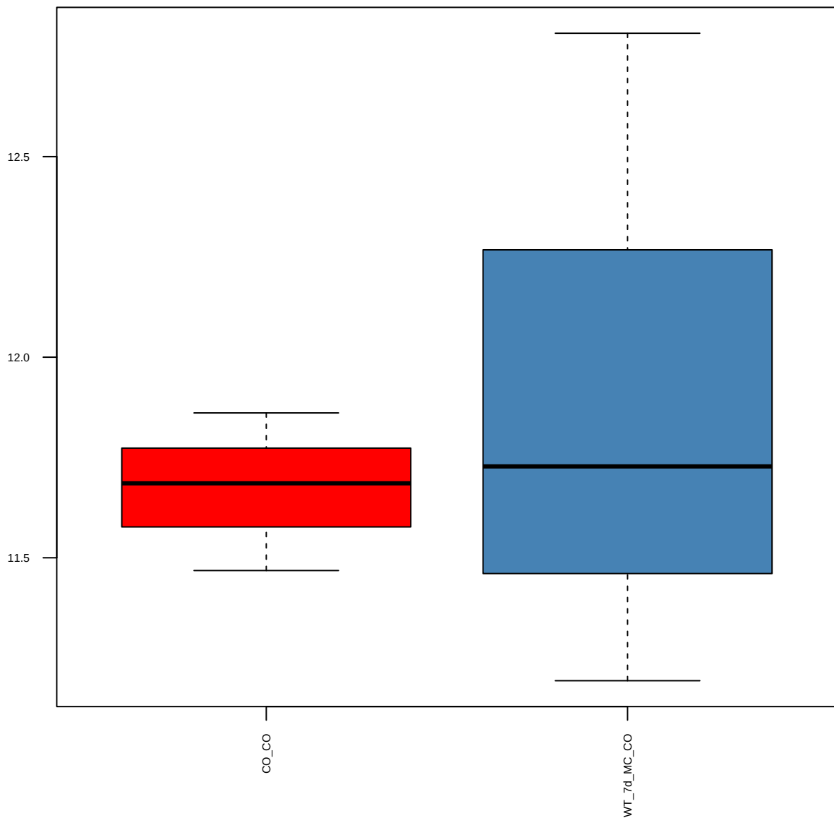
CD24(FL-80) (FDR = 1)
