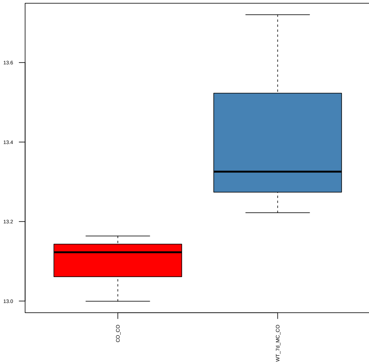
Stat3(D3Z2G) (FDR = 0.9)
