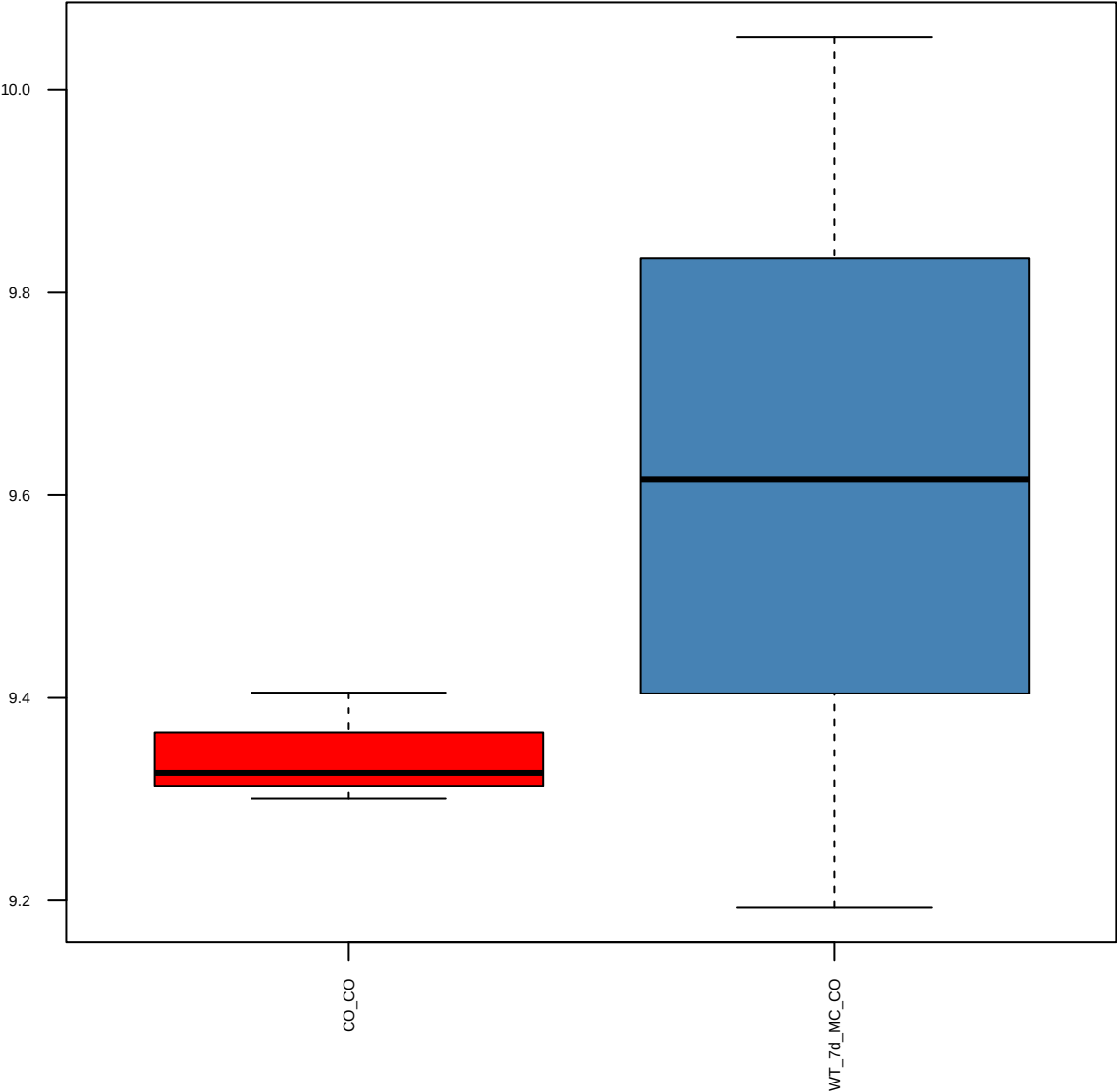
p-HER2/ErbB2(Y877) (FDR = 0.9)
