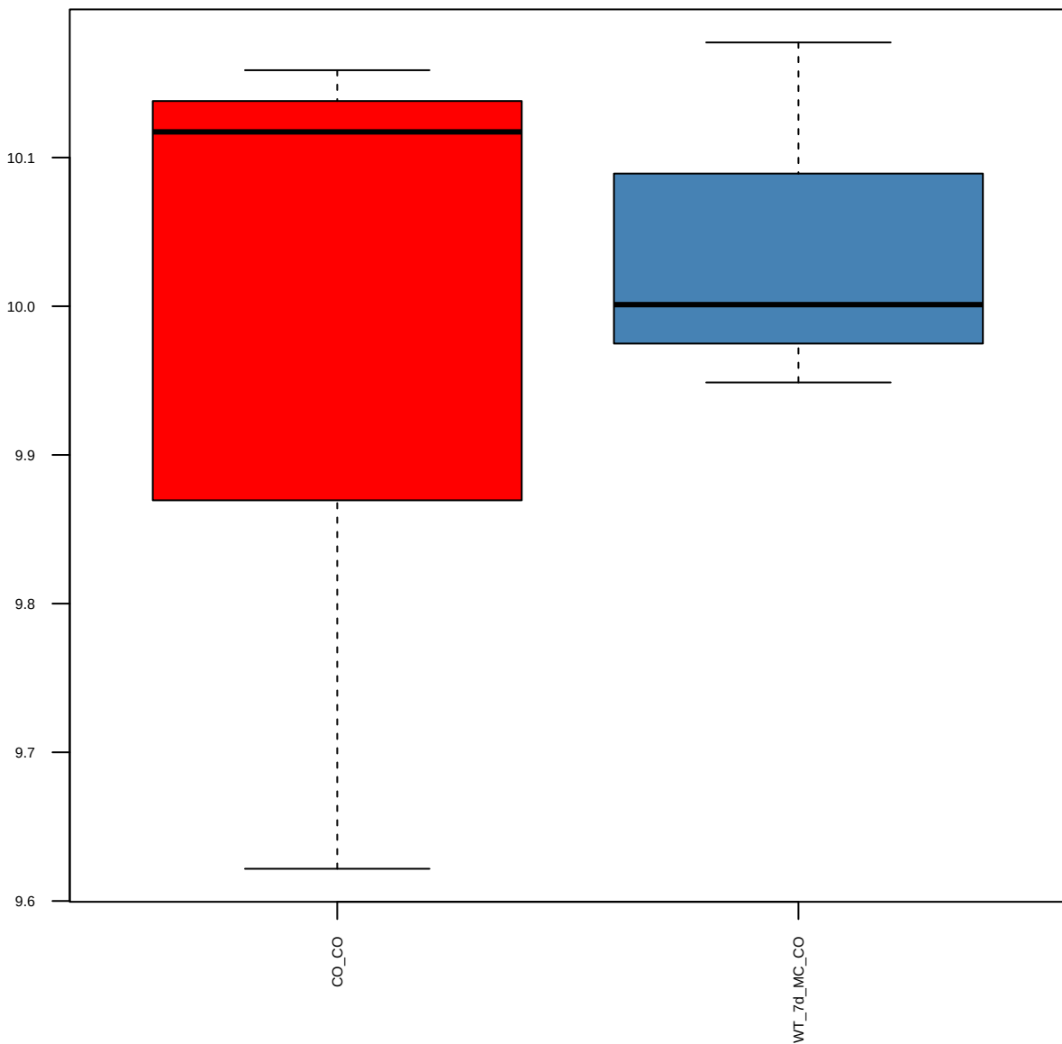
p-Beta-Catenin(S33/37/T41) (FDR = 1)
