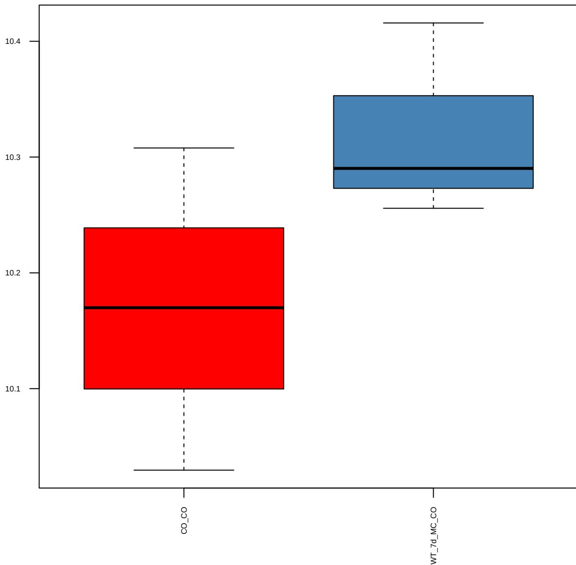
p-Caveolin-1(EPR2288Y)(Y14) (FDR = 0.9)
