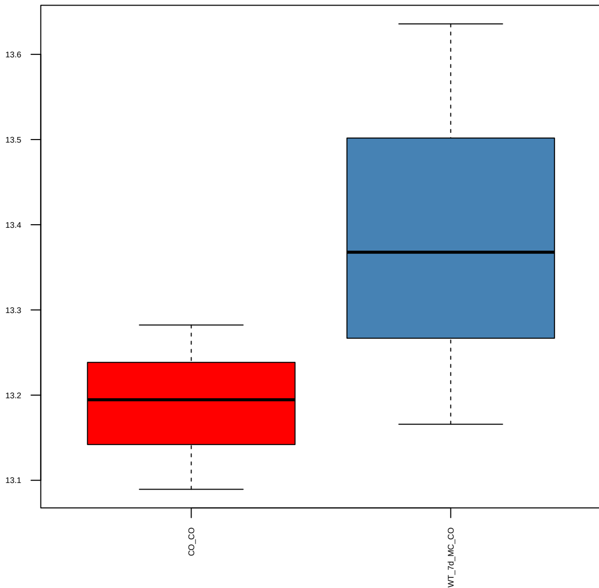
Stat5a(L-20) (FDR = 0.9)
