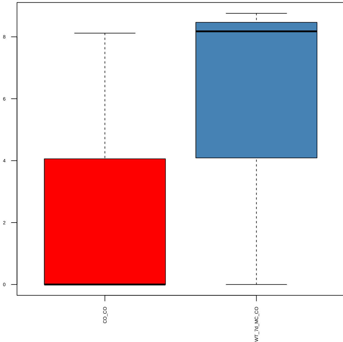
Beta-Catenin(CT) (FDR = 0.9)
