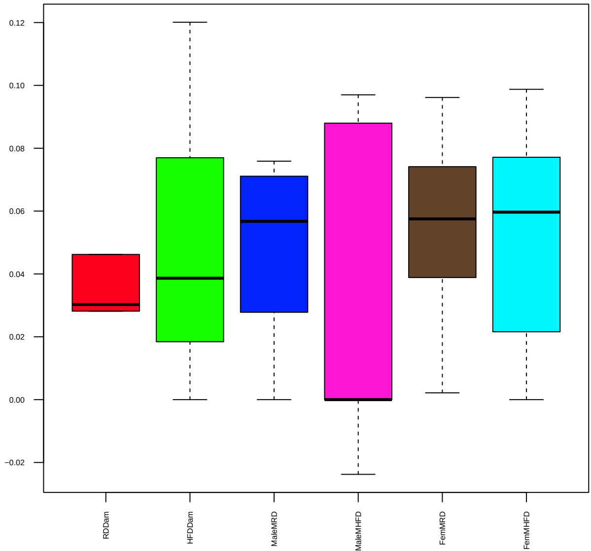
Serine (FDR = 0.94)
