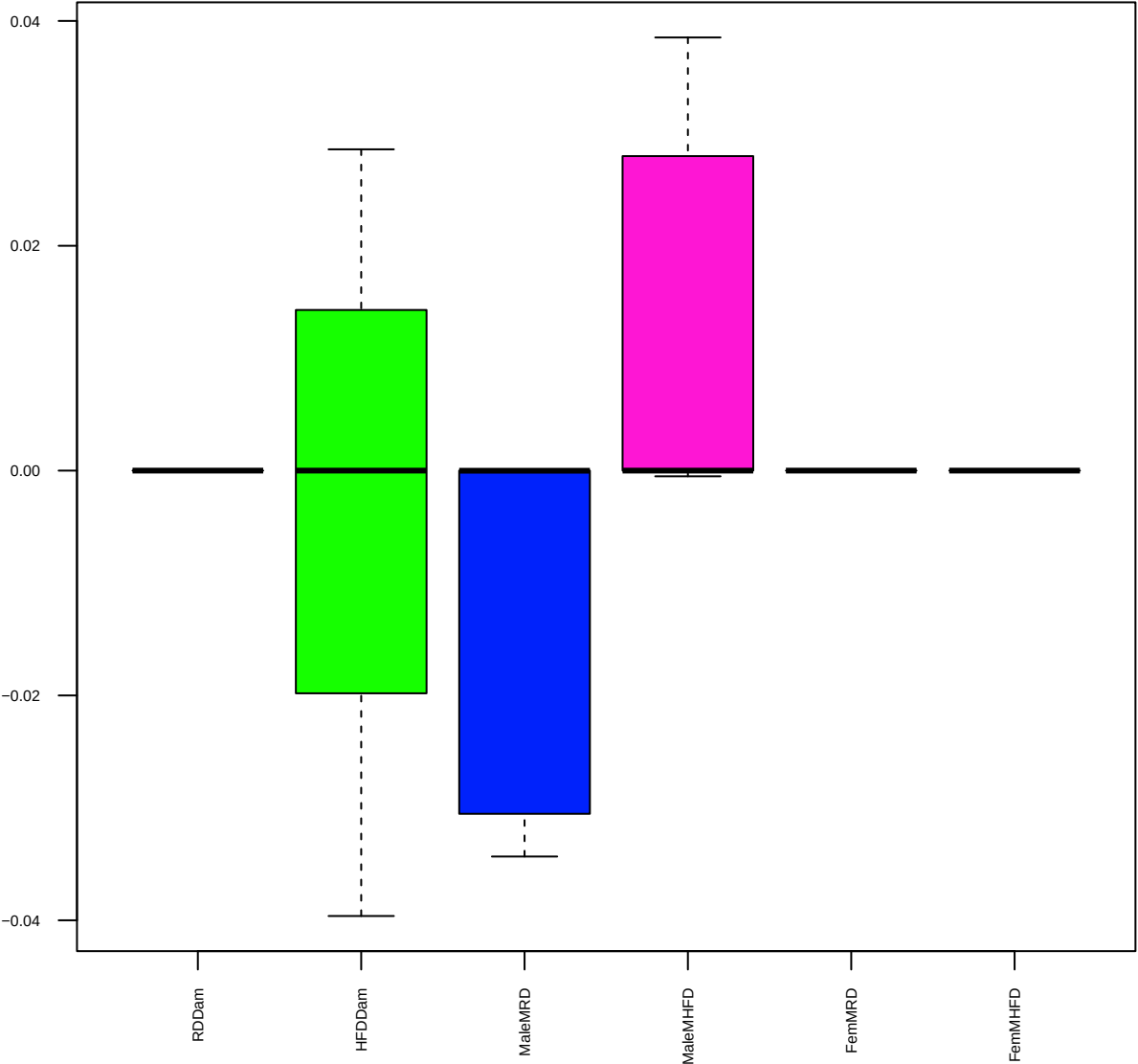
Proline (FDR = 0.53)
