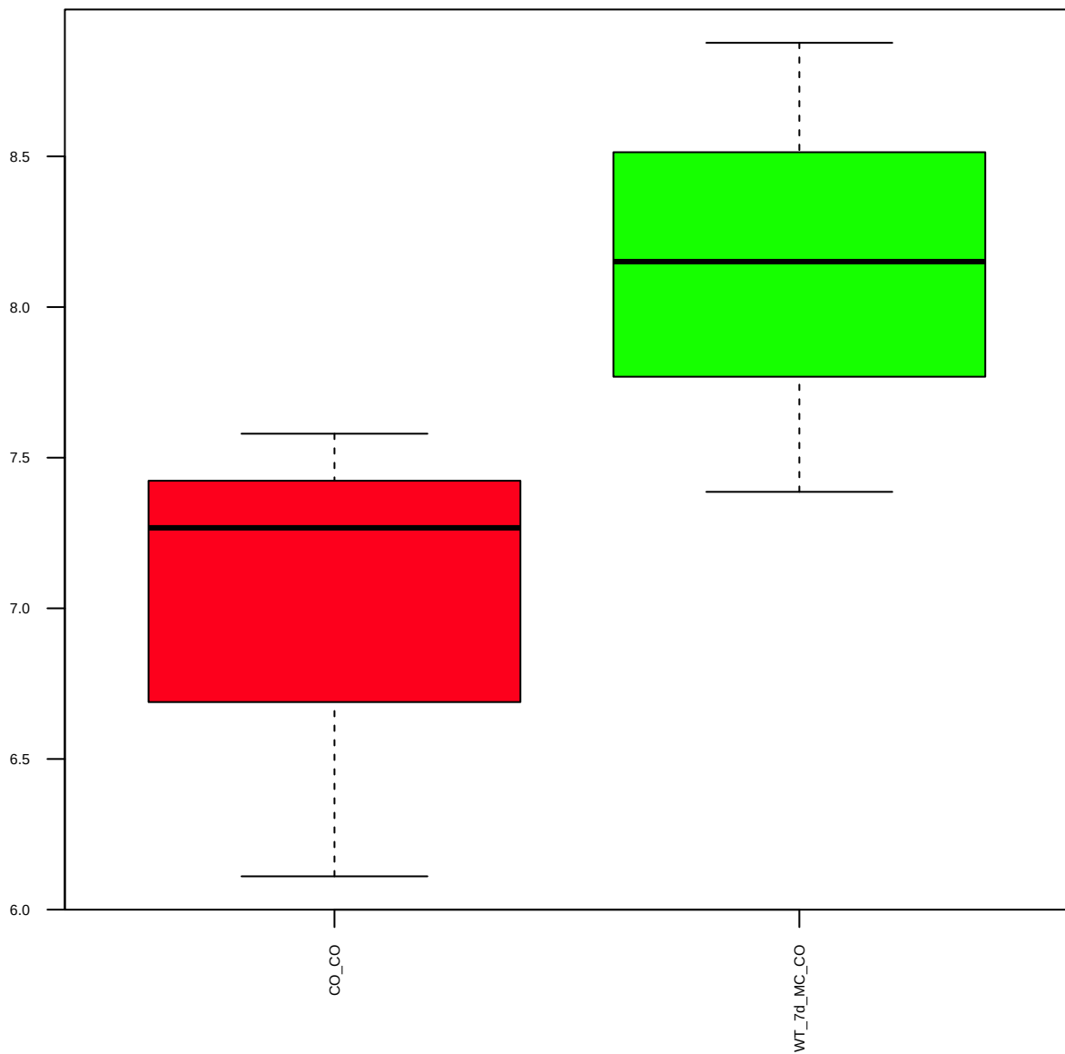
Atg12(D88H11) (FDR = 0.75)
