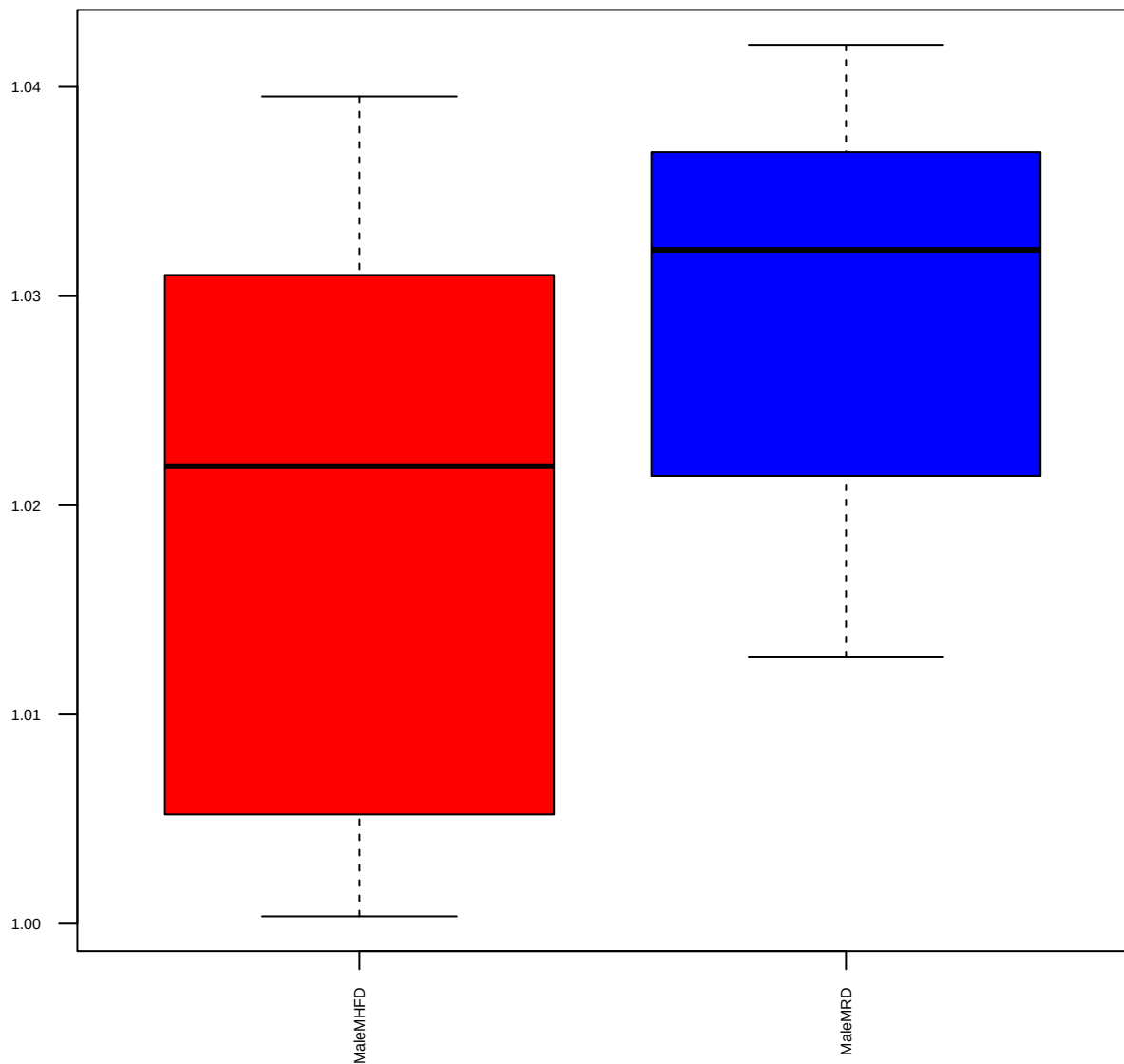
Citrulline (FDR = 0.48)
