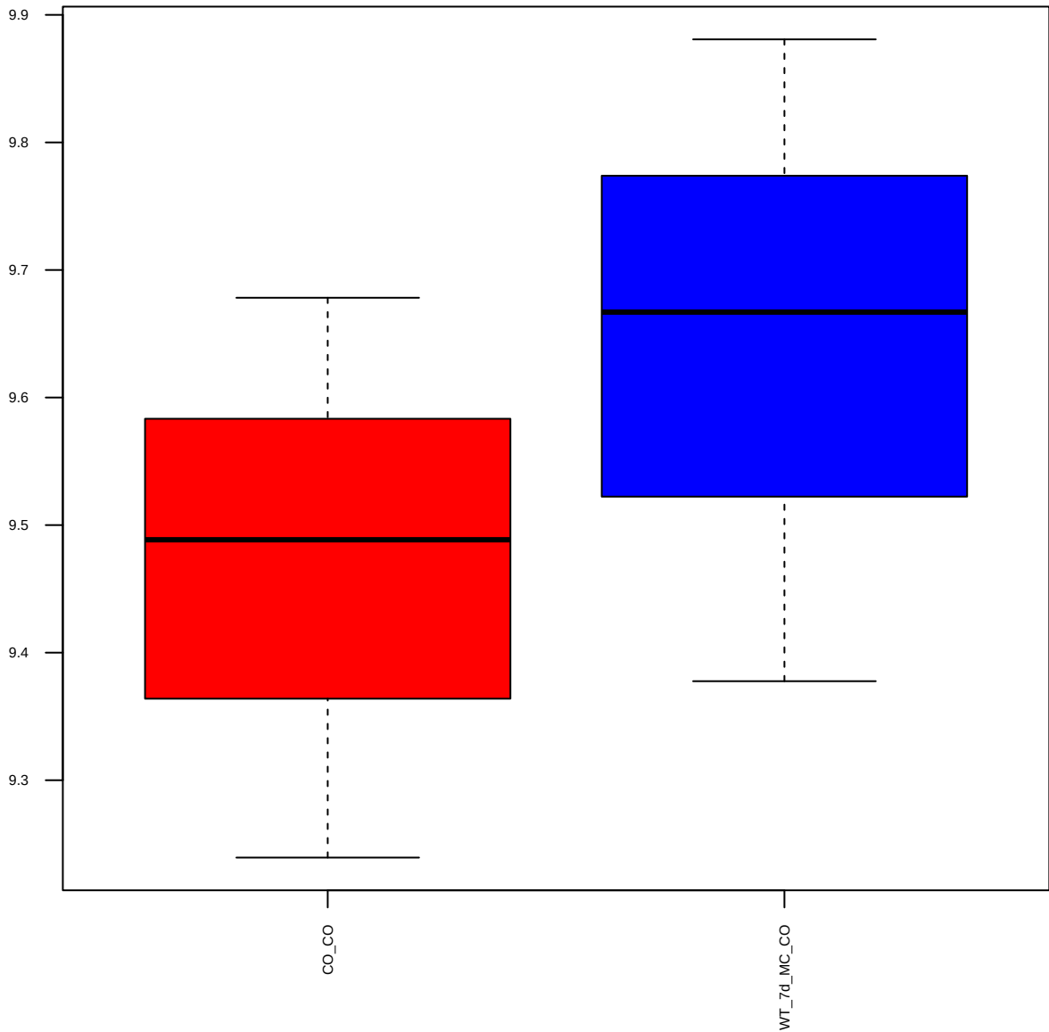
HDAC3 (FDR = 0.74)
