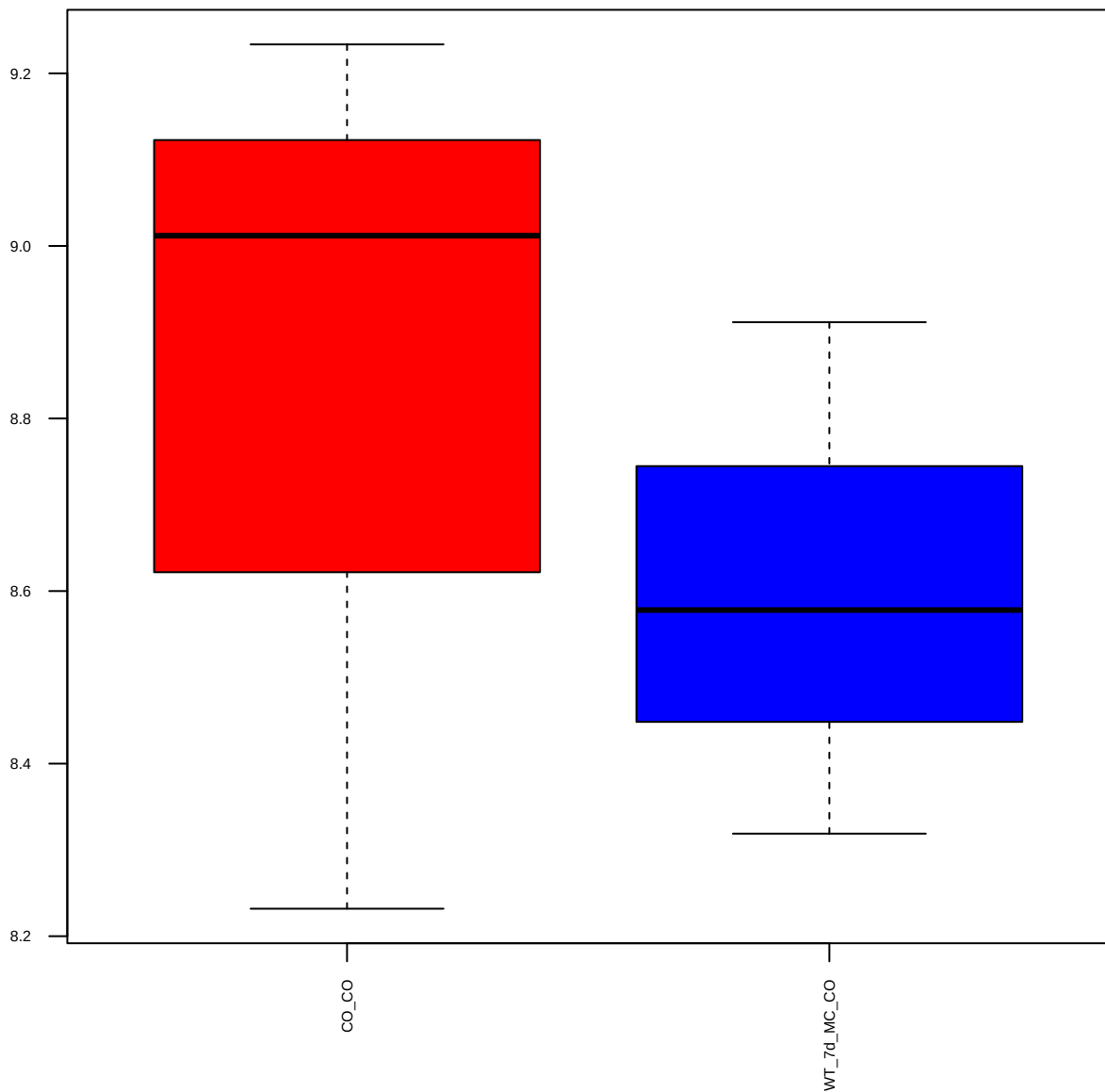
SMARCA1 (FDR = 0.79)
