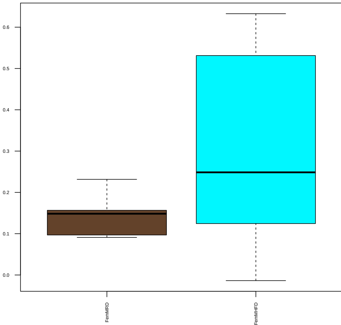
Serine (FDR = 0.81)
