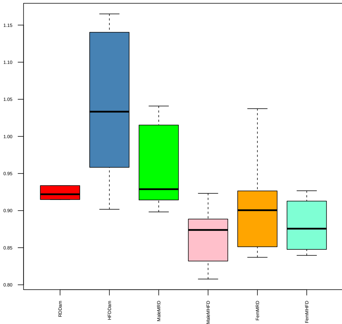
Glutamine (FDR = 0.01)
