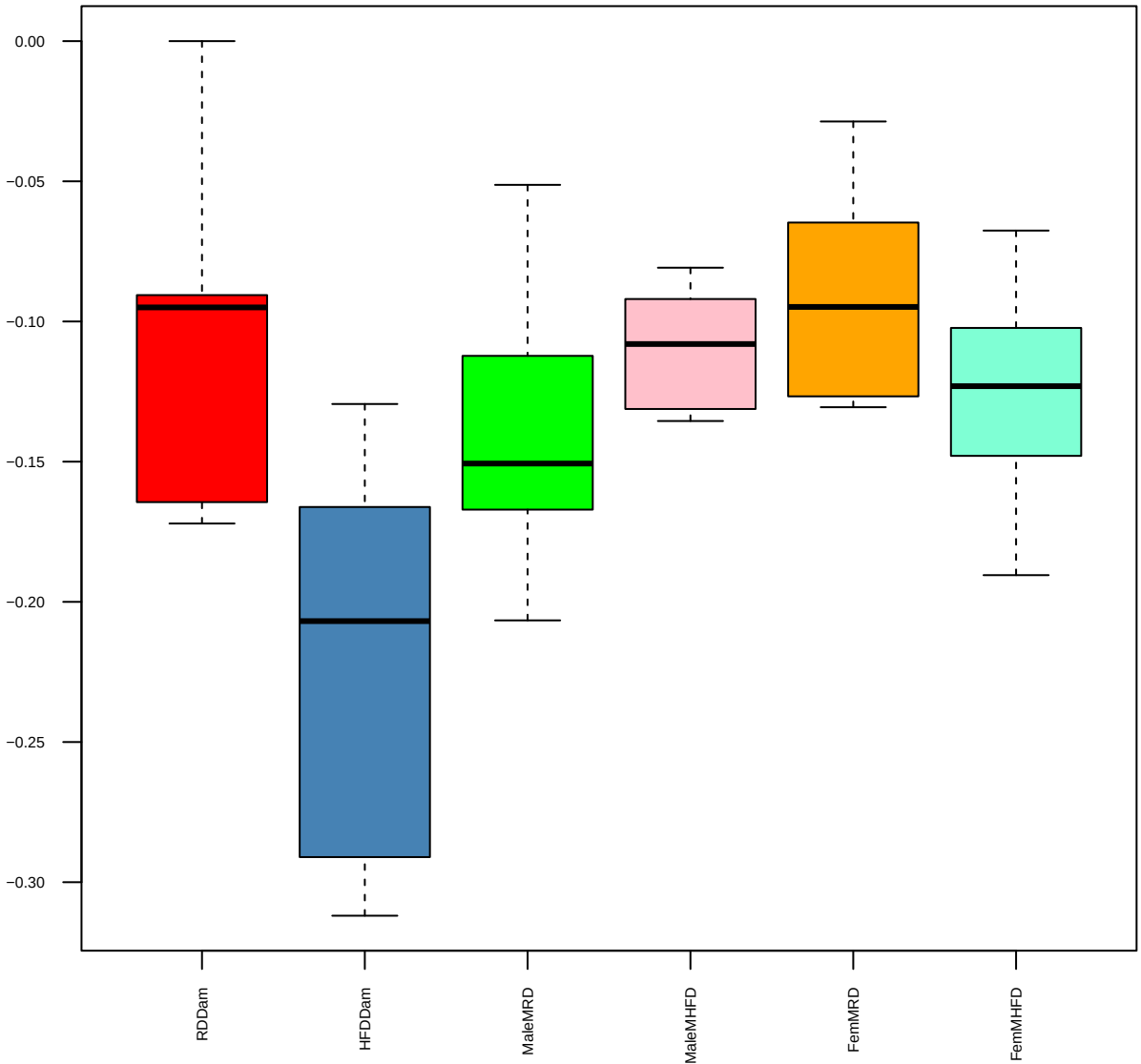
Methionine (FDR = 0)
