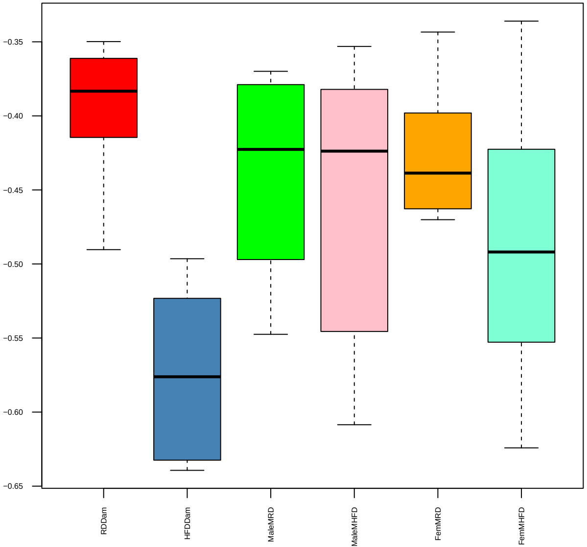
Alanine (FDR = 0.02)
