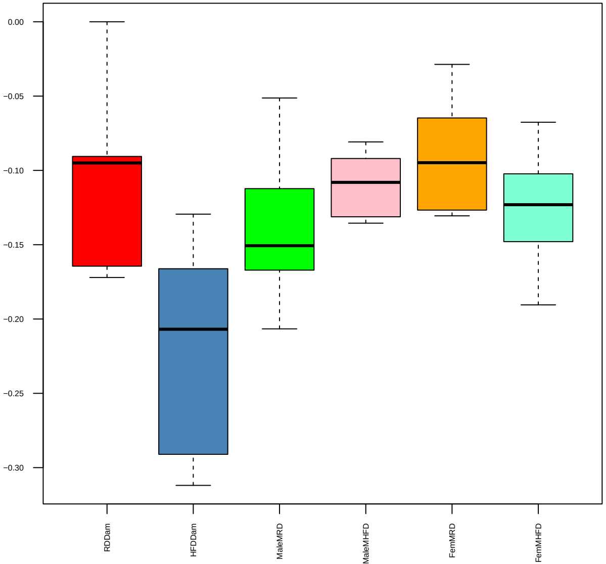
Methionine (FDR = 0)
