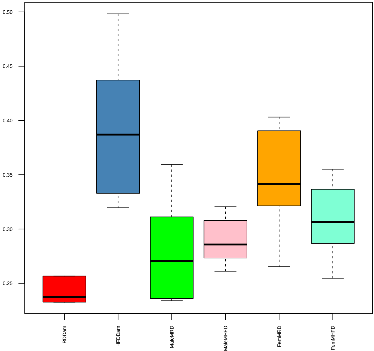
Valine (FDR = 0)
