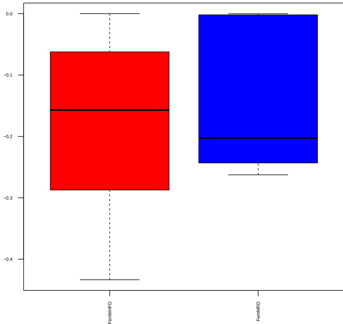
Cystine (FDR = 0.9)
