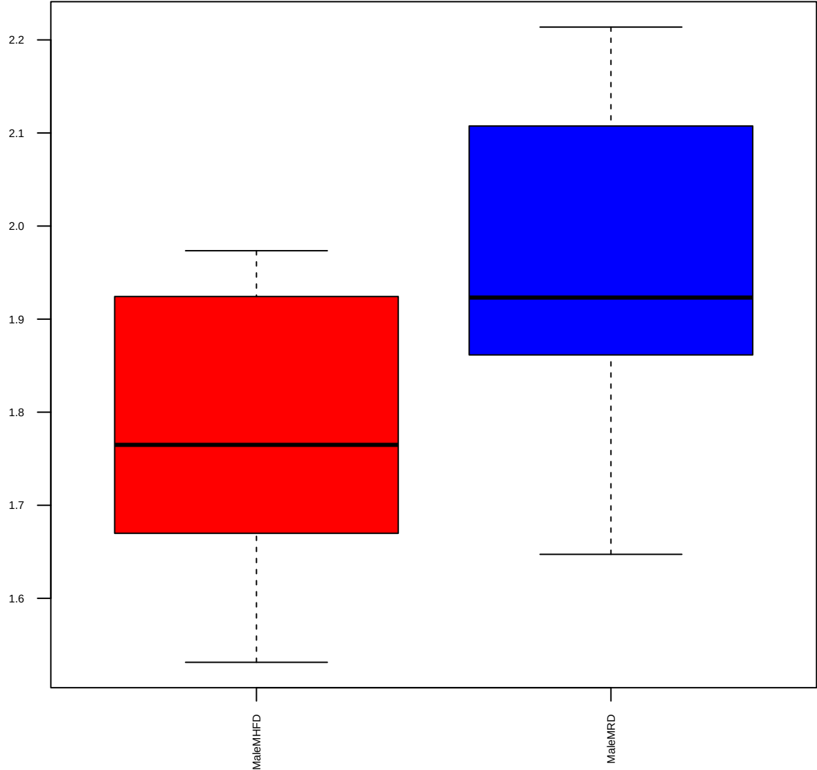
Histidine (FDR = 0.36)
