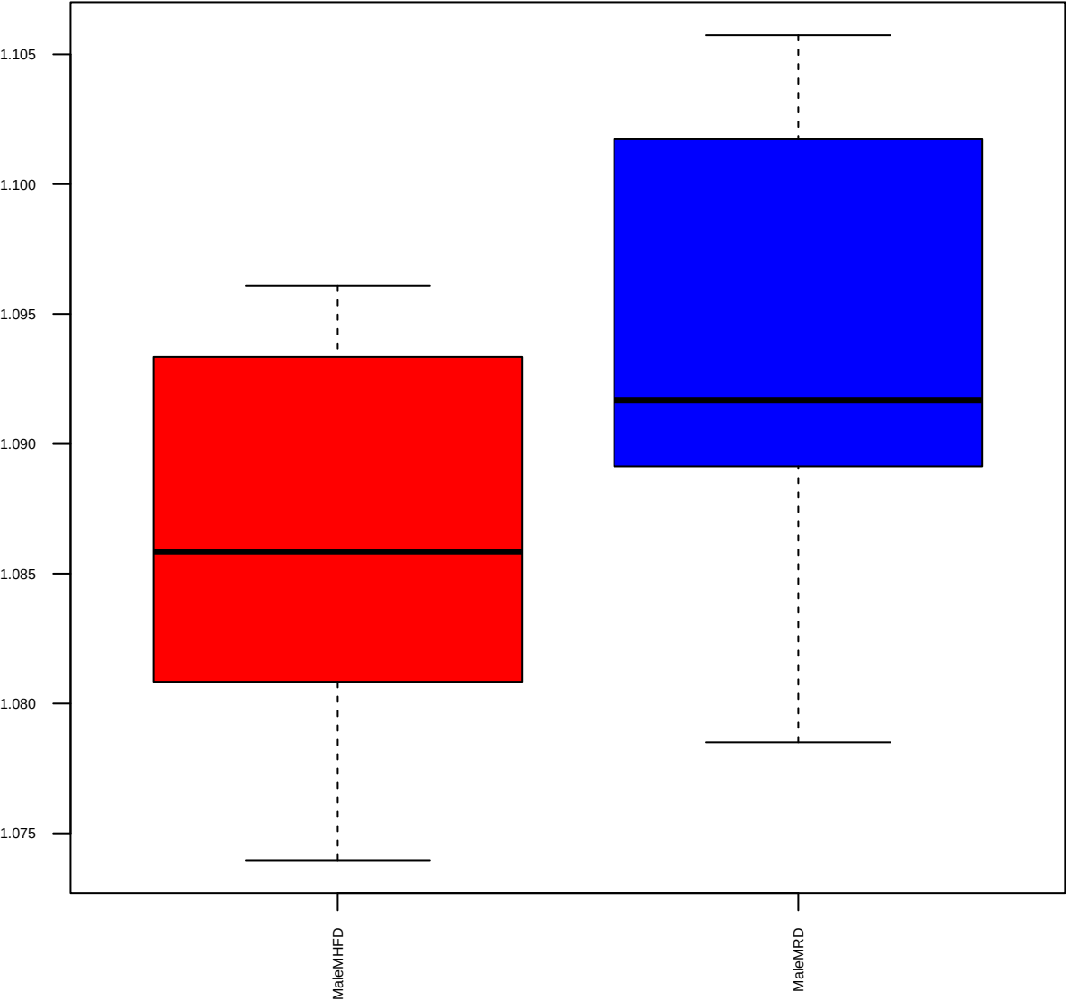
Histidine (FDR = 0.44)
