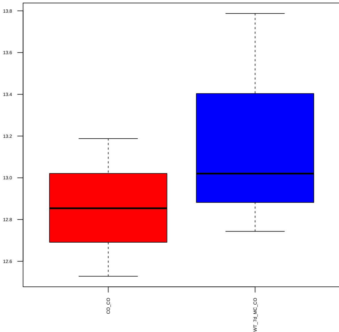
c-Src Antibody (B-12) (FDR = 0.9)
