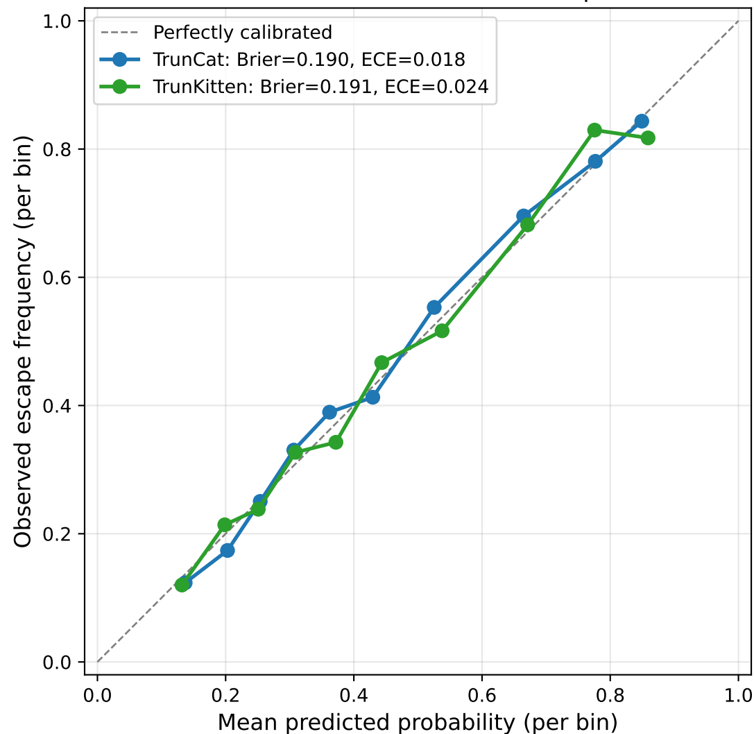
Calibration: TrunCat & TrunKitten OOF predictions
