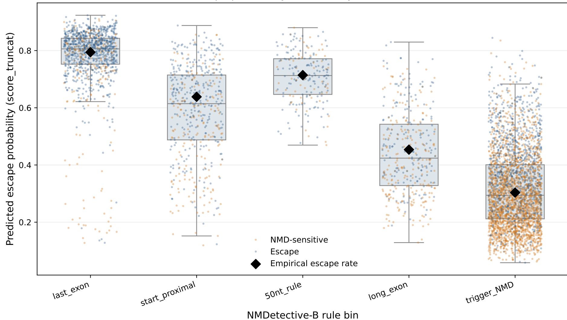
TrunCat escape probability stratified by NMDetective-B rule
