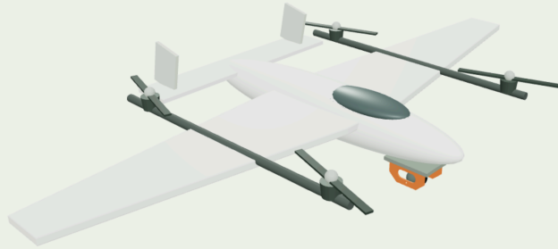
Sensor mount on a VTOL reference model · actual website CAD render
