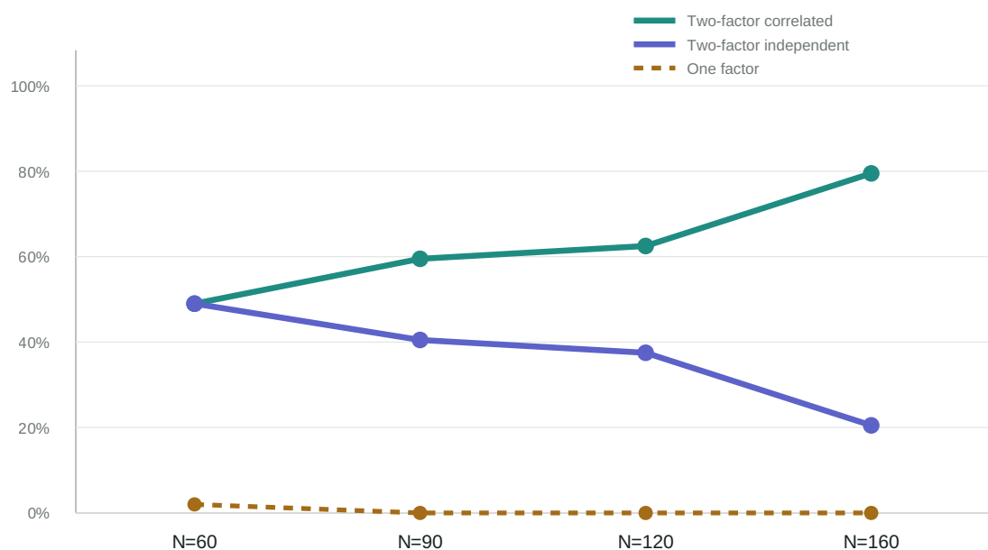
Figure 3 · Synthetic model-recovery diagnostic
