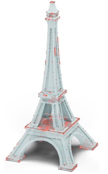
Fig. 5. Tangent points determined by short arcs (red dots) on a reconstructed Eiffel surface at n = 100^3 .
