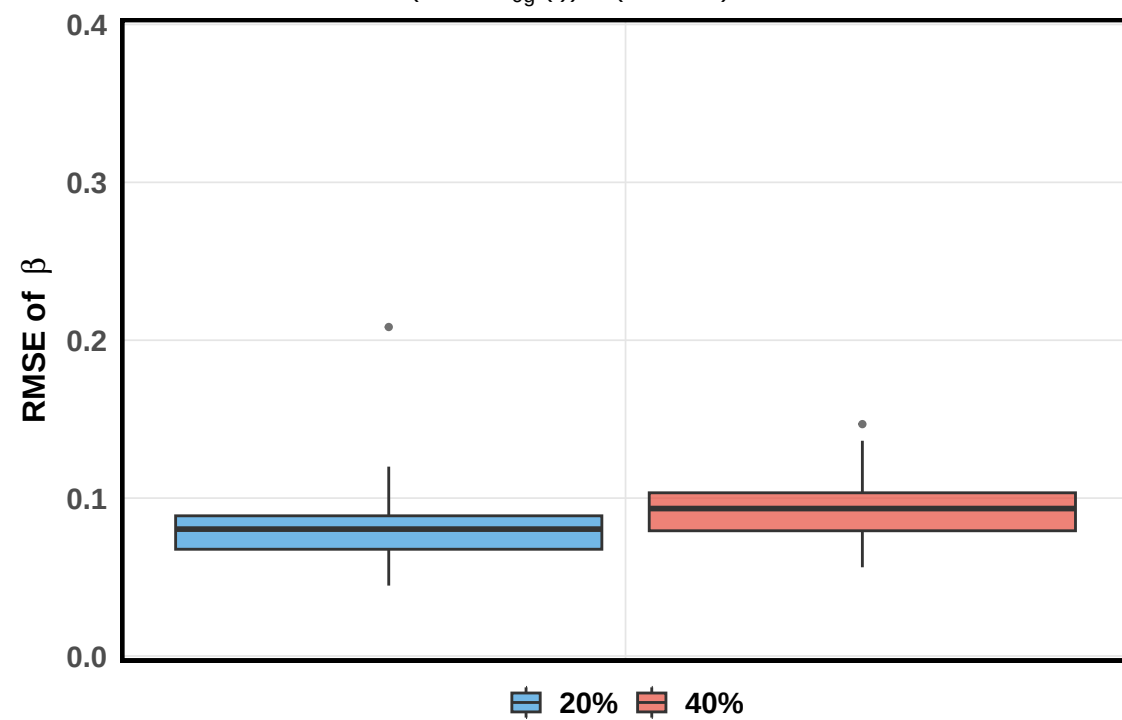
(J, G, \lambda_{0g}(t) ) = (35, 5, 1), N= 500
