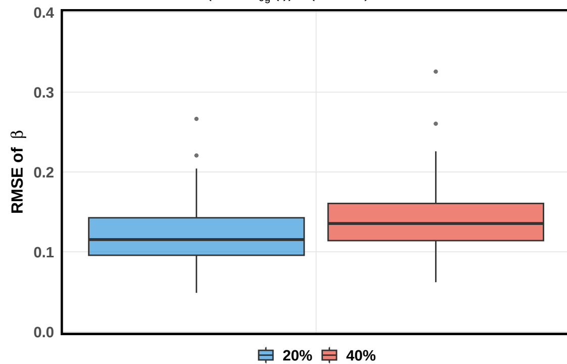
(J, G, \lambda_{0g}(t) ) = (25, 5, 1), N= 200
