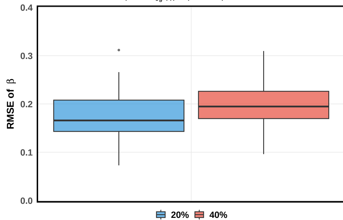
(J, G, \lambda_{0g}(t) ) = (15, 3, 2t), N= 200
