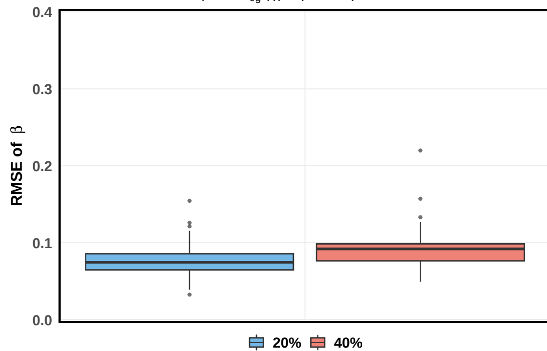
(J, G, \lambda_{0g}(t) ) = (15, 3, 2t), N= 500
