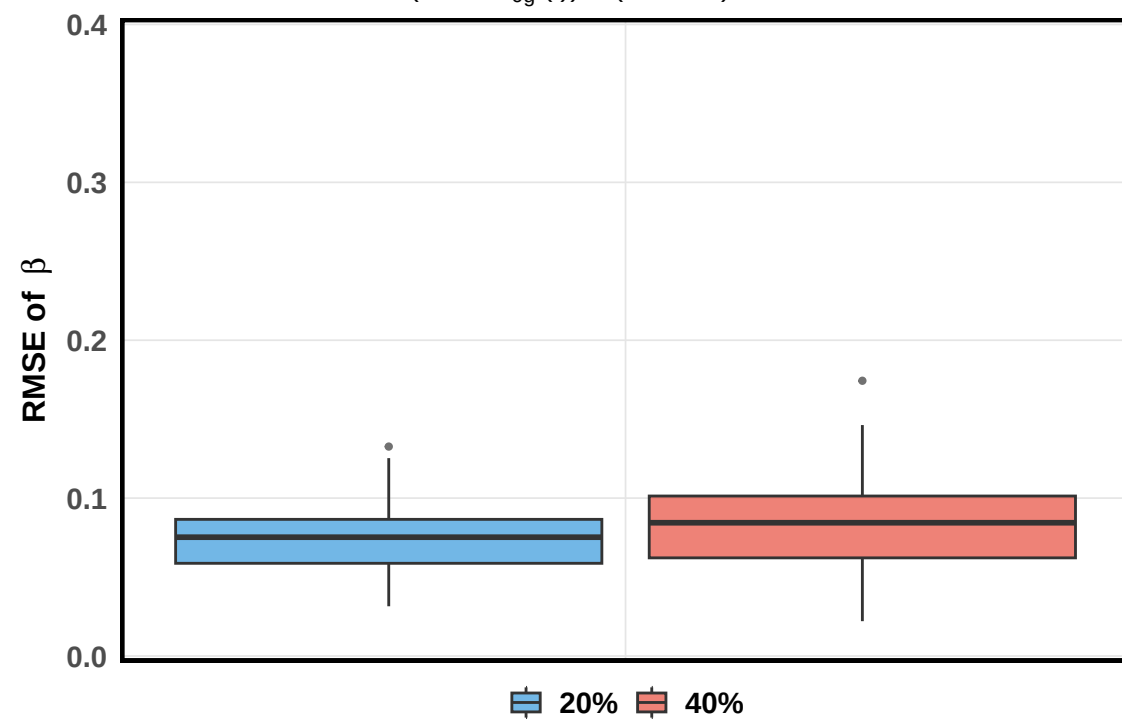
(J, G, \lambda_{0g}(t) ) = (25, 5, 1), N= 500
