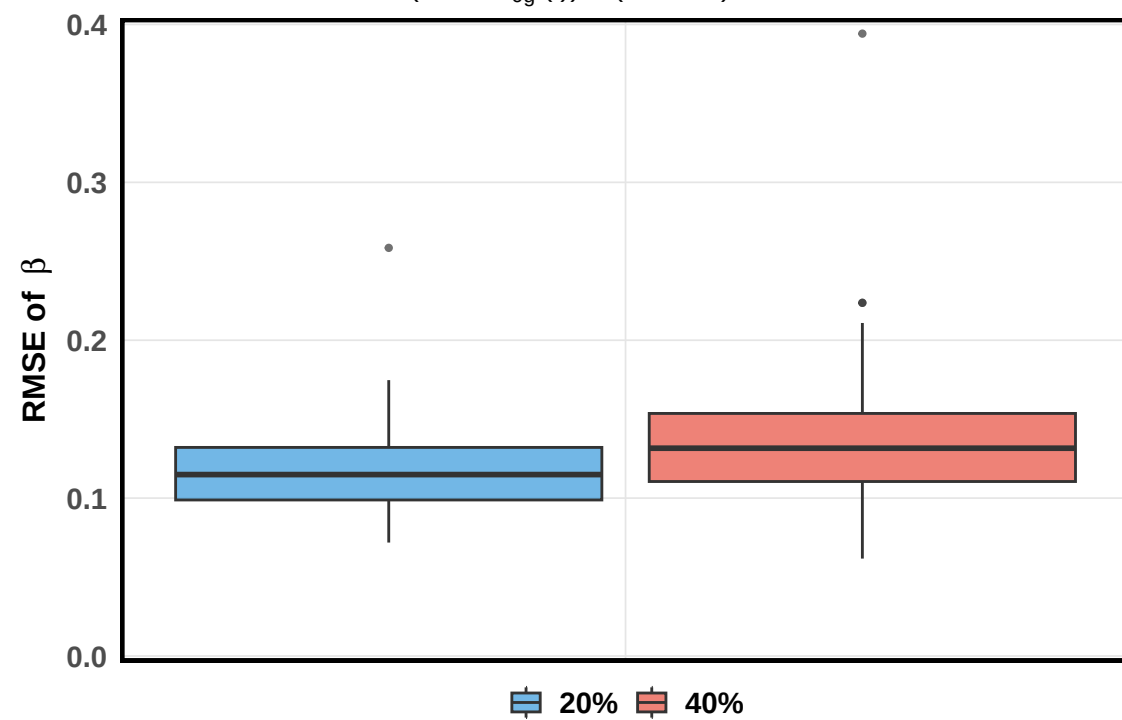
(J, G, \lambda_{0g}(t) ) = (35, 5, 1), N= 200
