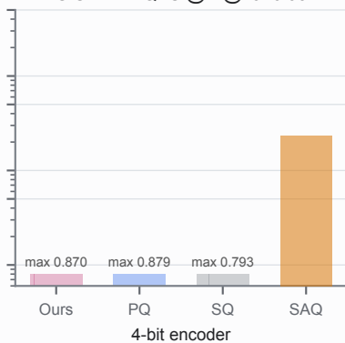
b GIST-1M · QPS @ R@10=0.95
