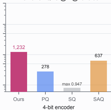
c AGNews · QPS @ R@10=0.95
