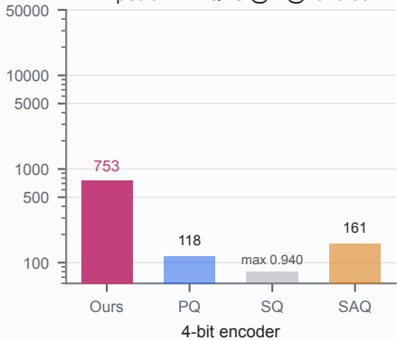
a DBpedia-1M · QPS @ R@10=0.95
