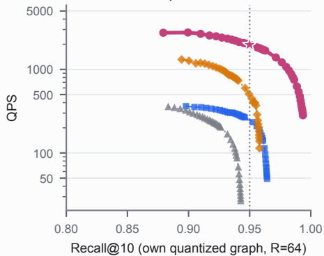
DBpedia-1M
