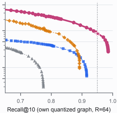
GIST-1M
