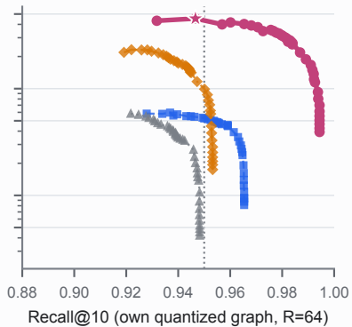
AGNews
