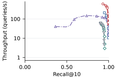
(a) AGNews
