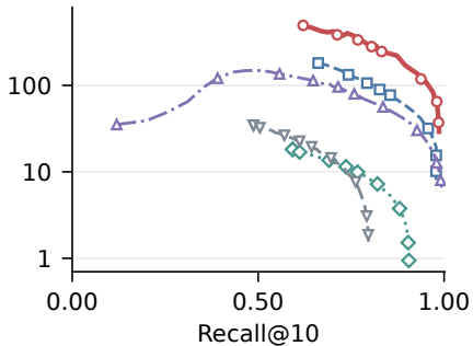
(b) GIST
