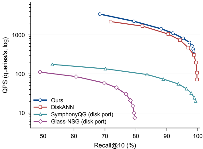
GIST | all four disk systems | log QPS axis
