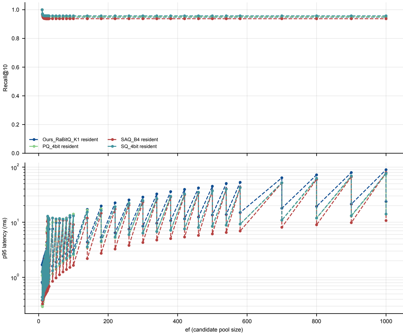
05A agnews: fixed-candidate recall / latency vs ef (dev/smoke)
