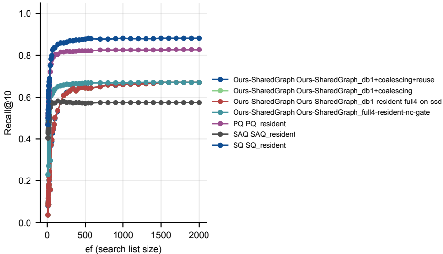
05B gist: shared-graph disk search vs ef (dev/smoke)
