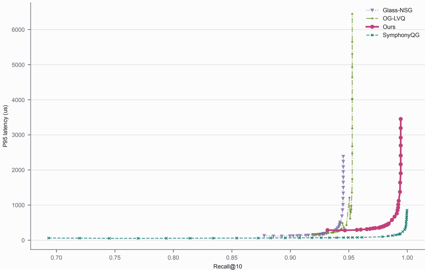
Recall@10 vs P95 latency · Ours uses DB1 × INT8 query
