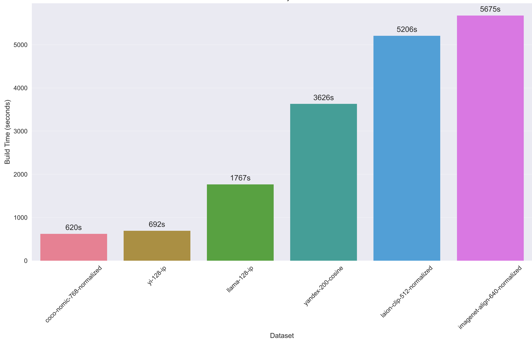
Build Time by Dataset
