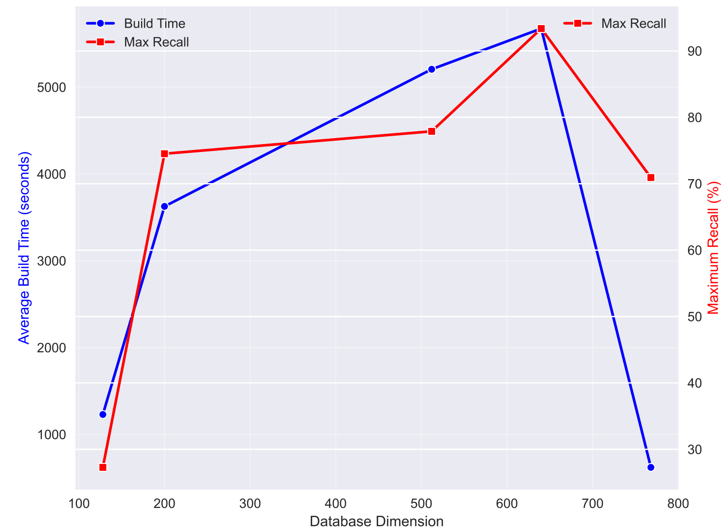
Performance vs Database Dimension
