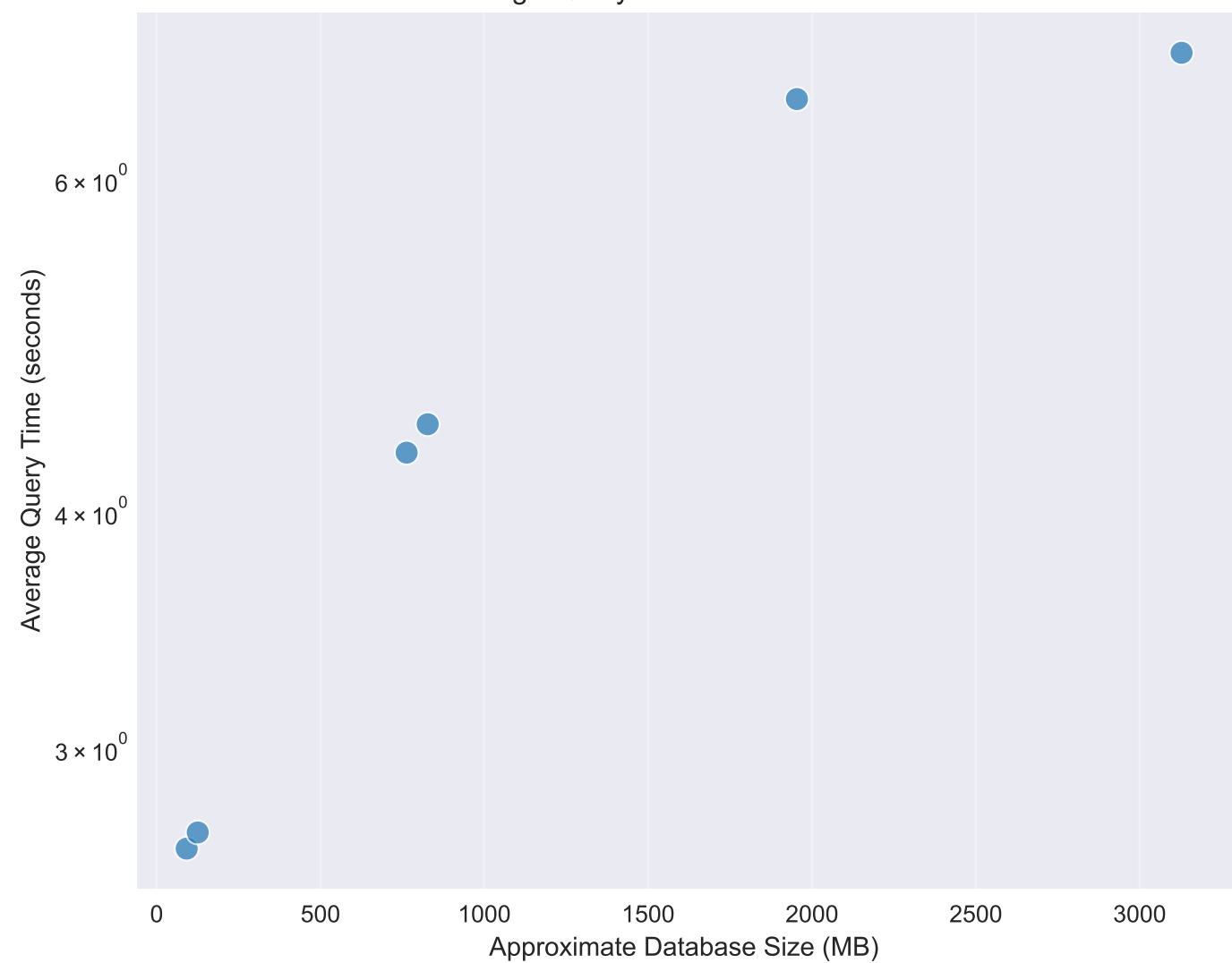
Performance vs Database Dimension
