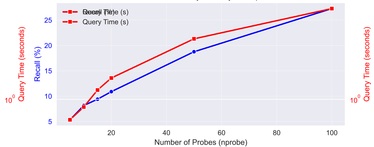
Recall vs Query Time - yi-128-ip
