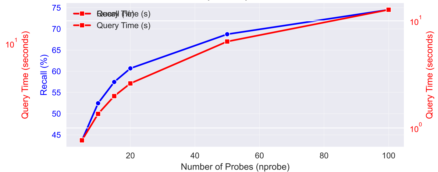
Recall vs Query Time - laion-clip-512-normalized
