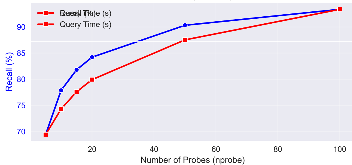
Recall vs Query Time - coco-nomic-768-normalized
