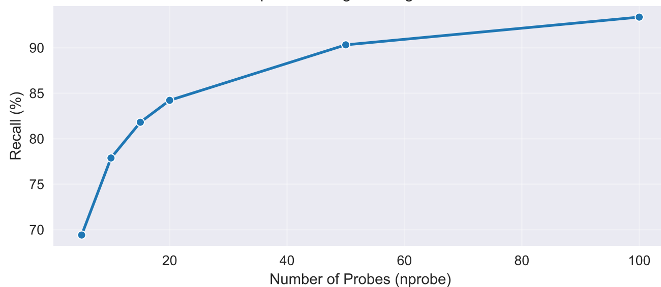
Recall vs nprobe - coco-nomic-768-normalized
