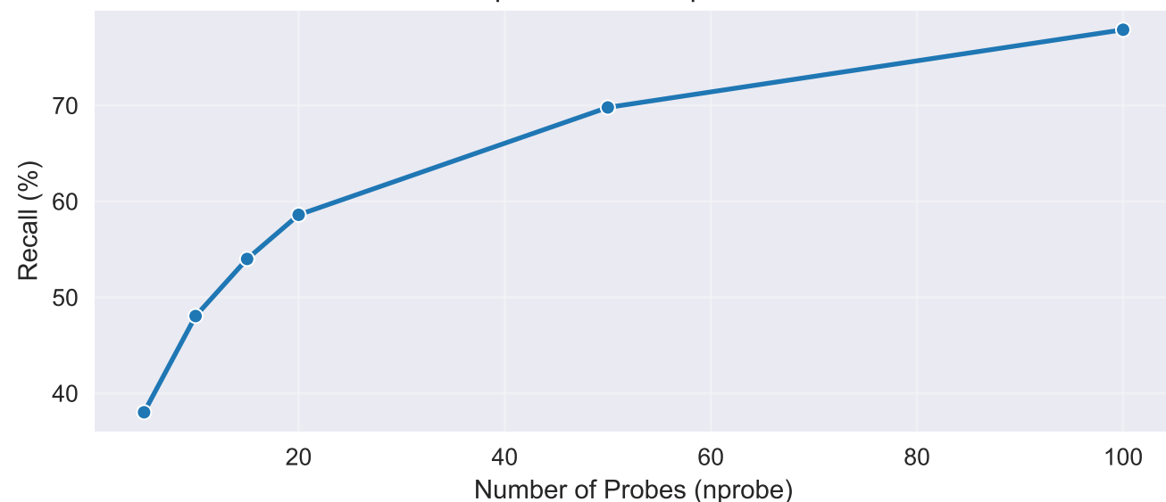
Recall vs nprobe - yi-128-ip
