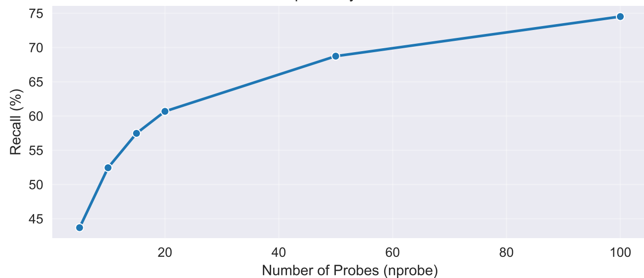
Recall vs nprobe - laion-clip-512-normalized
