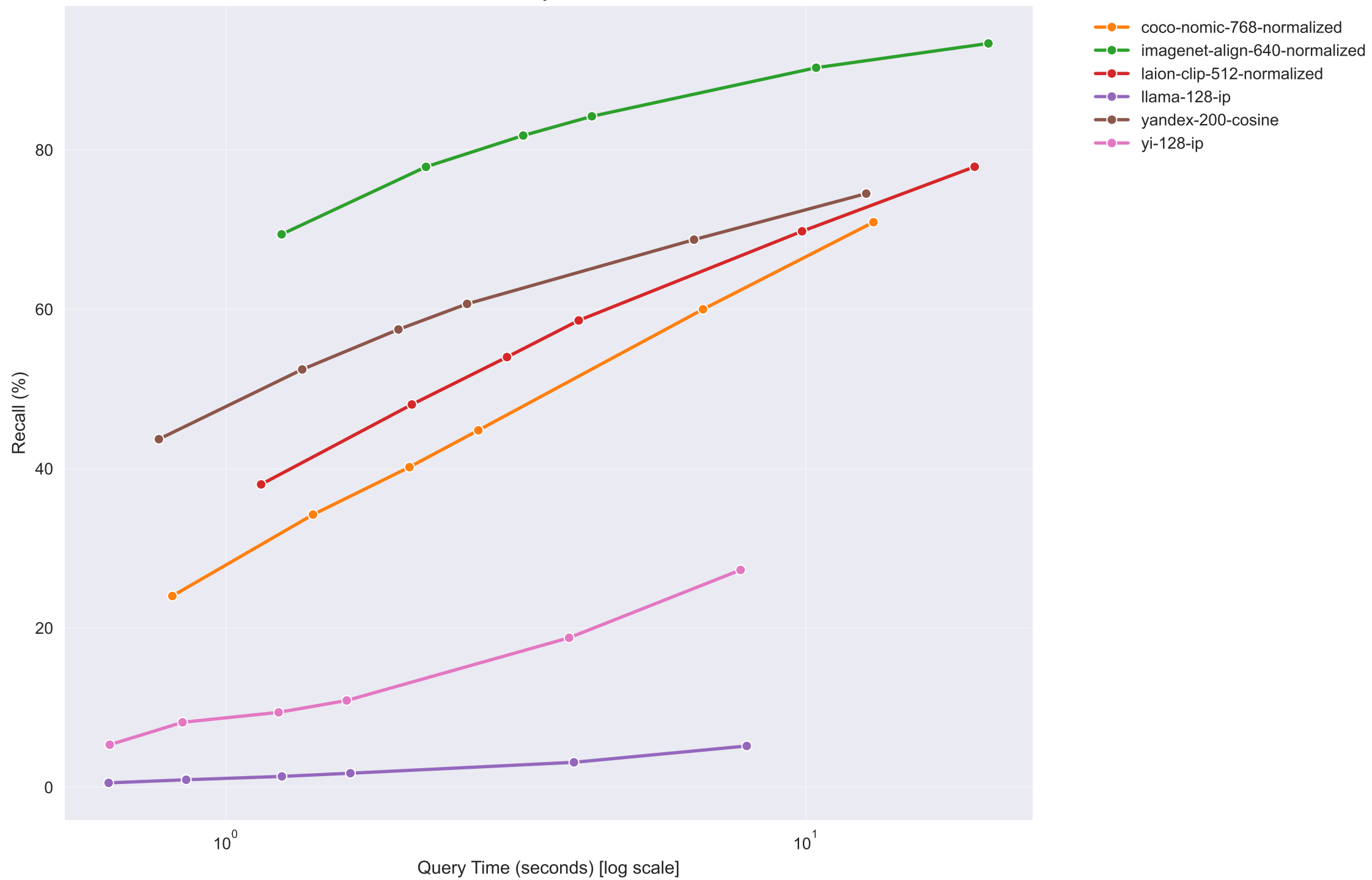
Recall vs Query Time Trade-off
