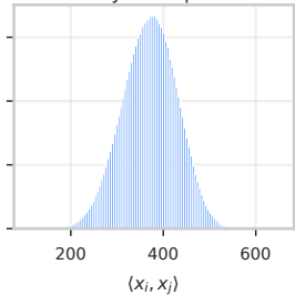
yi-128-ip
