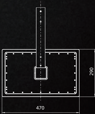
Wall Hung Overhead Shower 入牆式花灑
