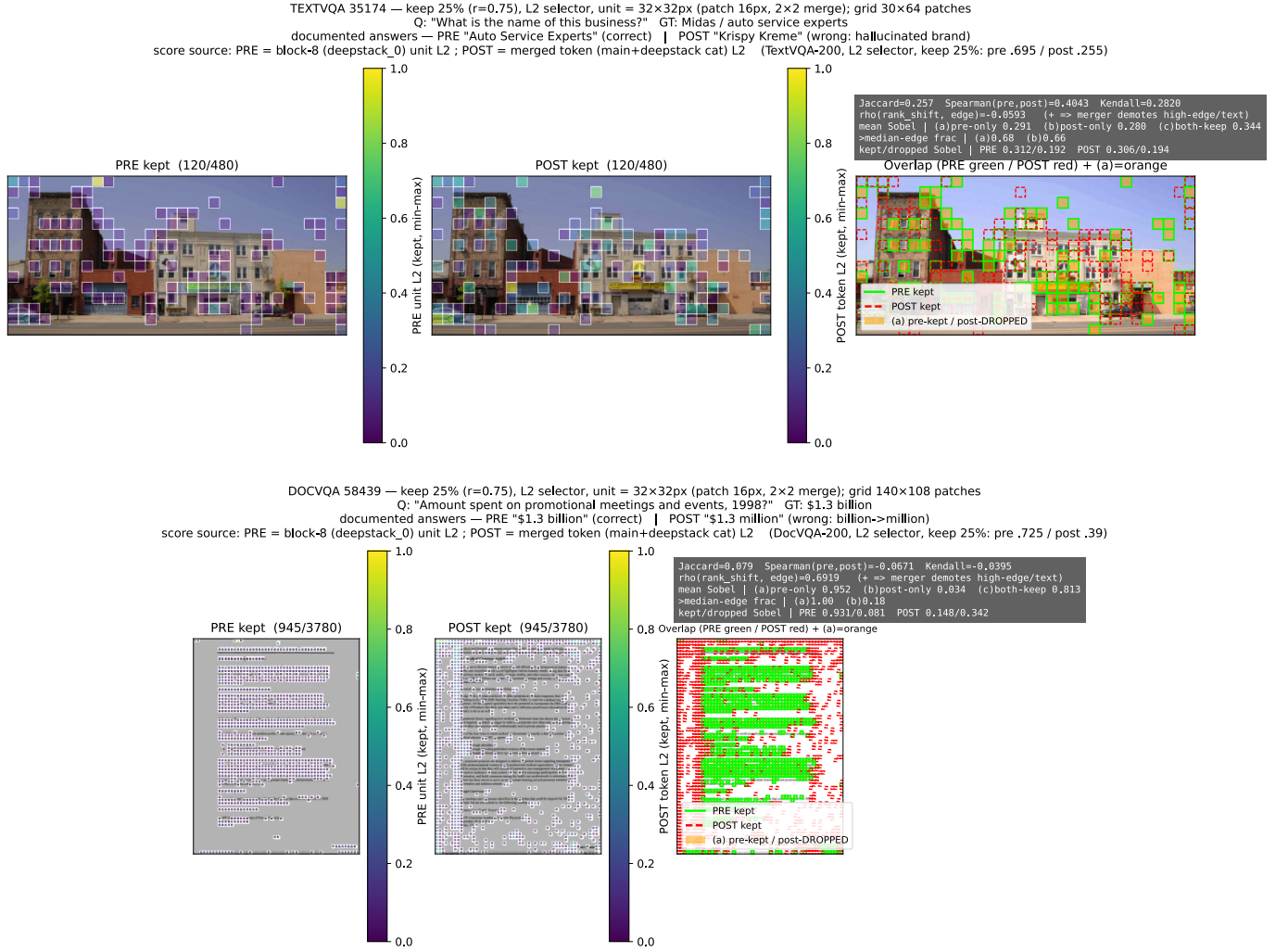
Fig. 1. Representative token-survival maps at 25% retention. TextVQA (top) and DocVQA (bottom) use the same query-blind L2 selector before and after Qwen3-VL's native merger. In each row, the first two panels show the pre- and post-selected units; the third overlays pre-kept (green), post-kept (red dashed), and pre-only/post-dropped units (orange). These are audited single-image mechanism examples, not aggregate accuracy evidence.
