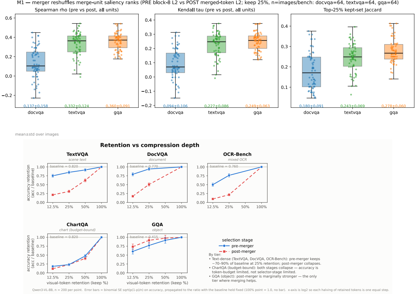
Fig. 2. Quantitative mechanism and depth diagnostics. Top: per-image pre/post rank agreement on the deterministic seed-0 M1 sample ( n = 64 per benchmark); boxes and points show the distributions, with mean±standard deviation annotated. Bottom: normalized accuracy as compression deepens on Qwen3-VL-8B ( n = 200 per point). Pre-merger selection preserves substantially more text-dense accuracy, while ChartQA is primarily budget-limited and GQA does not exhibit the text-dense stage effect. Error bars are descriptive rate-approximation standard errors; primary inference uses paired metric-level bootstrap and sign-flip tests.
