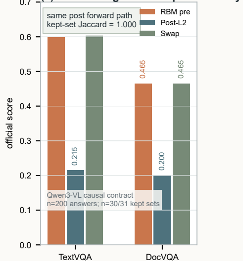
(c) Pre ranking recovers pre accuracy
