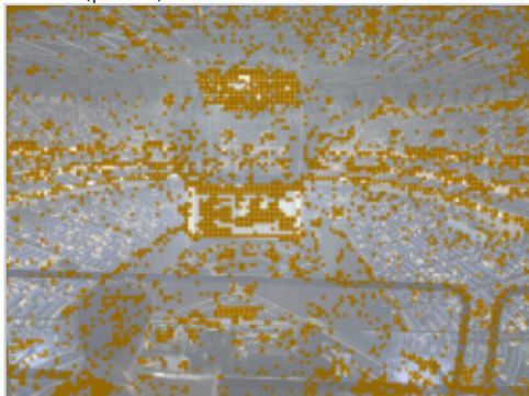
b RBM (pre L2)
