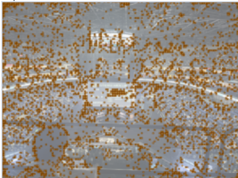
c post L2
