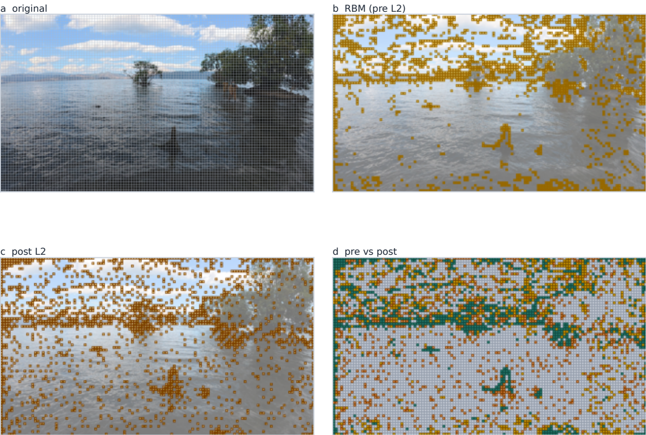
N=8160 k=2040 (25% kept) top-k Jaccard=0.3377 Spearman \rho(\text{pre, post ranks})=0.3963 unit grid 68 \times 120 = \text{grid\_thw}/2 Qwen3-VL-8B measured merger L2 FastV: SKIPPED (no user question; inputs/manifest.json absent) (a) full unit grid outline (light). (b,c) SAME amber L2 selector & 25% budget; (c) hatched = post (distinguishable without color). (d) four states kept-by-both / RBM-only / post-only / dropped-by-both, encoded by color + hatch/outline (legend). ■ kept by both (pre & post) ■ RBM-only (pre & ~post) ■ post-only (~pre & post) ■ dropped by both
