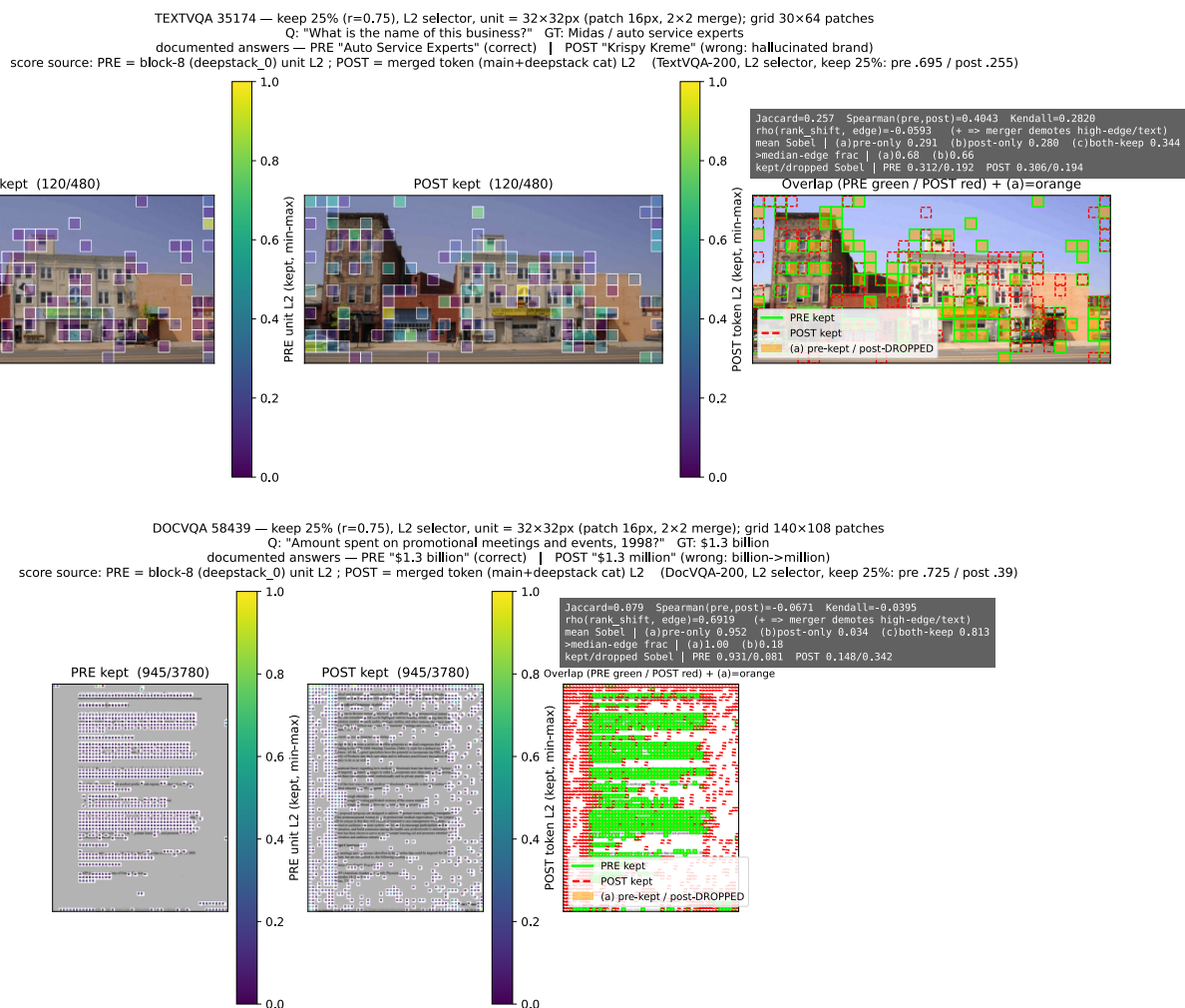
Figure 4: Representative token-survival maps at 25% retention. TextVQA (top) and DocVQA (bottom) use the same query-blind L2 selector before and after Qwen3-VL’s native merger. In each row, the first two panels show the pre- and post-selected units; the third overlays pre-kept (green), post-kept (red dashed), and pre-only/post-dropped units (orange). These are audited single-image mechanism examples, not aggregate accuracy evidence.
