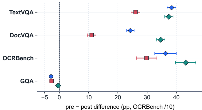
(a) Operational RBM vs Post-L2
