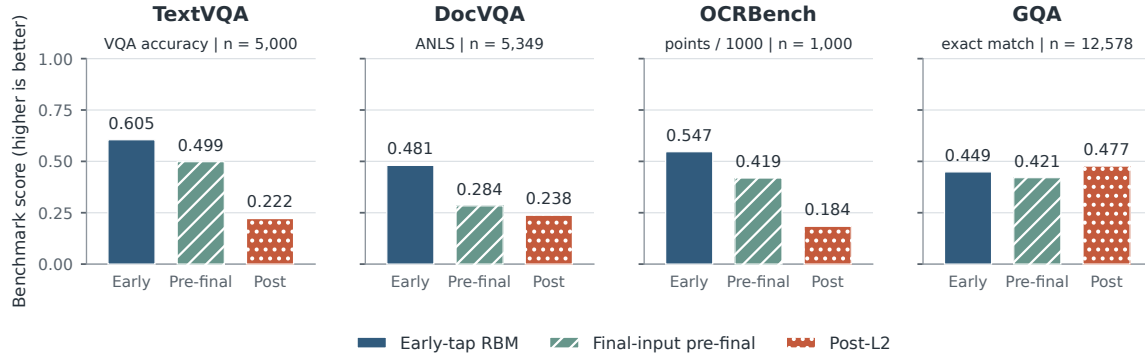
Figure 2: Full-split Qwen3-VL accuracy at 25% retention. Early-tap RBM is the operational design; Pre-final and Post-L2 form the stricter final-input comparison. OCRBench is normalized by 1,000. The RBM–Pre-final difference also includes auxiliary-stream handling and is not a feature-depth-only intervention.
