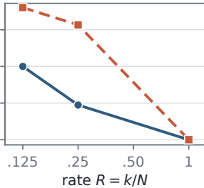
OCRBench
