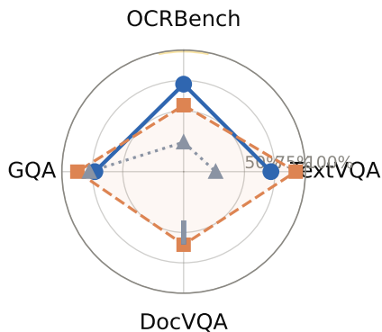
(c) OCR regime: accuracy vs visual tokens OCRBench; RBM = home regime
