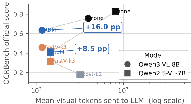
(c) OCR regime: accuracy vs visual tokens OCRBench; RBM = home regime
