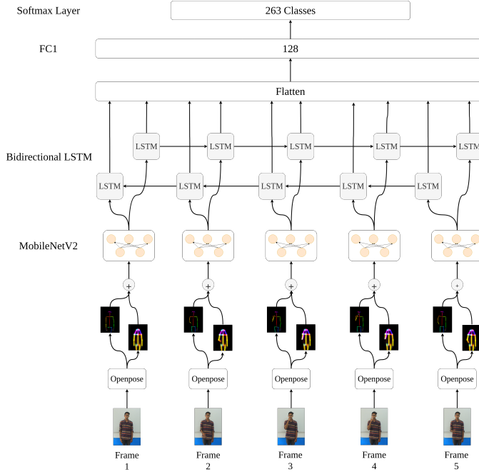
Figure 2: Model pipeline for Method 2 - Each frame is passed through OpenPose and the Pose and PAF videos are obtained. A channel-wise concatenation is done and fed through MobileNetV2 model to extract features. The extracted features are fed to a BiLSTM. The hidden states from LSTM cells are flattened and passed through a fully connected layer and a softmax layer for classification.
