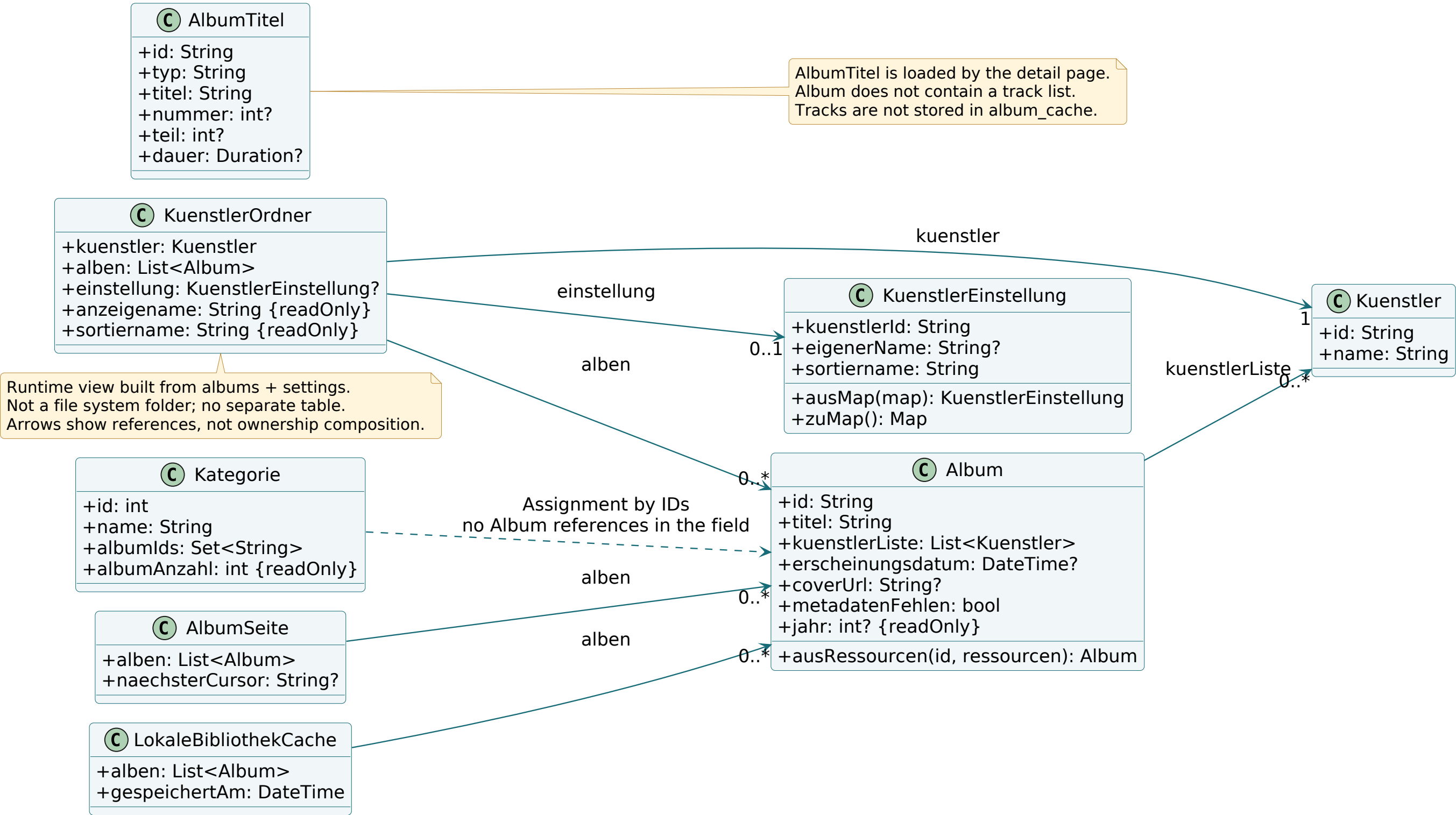
Domain models in memory
