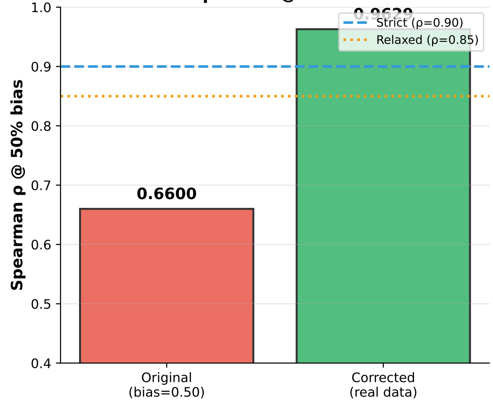
Comparison @ 50% Bias
