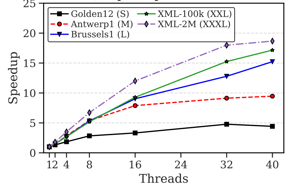
(f) Speedup vs. Threads
