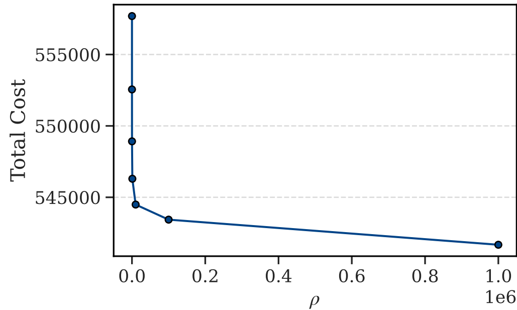
(a) Cost vs. \rho : Brussels1 (L)
